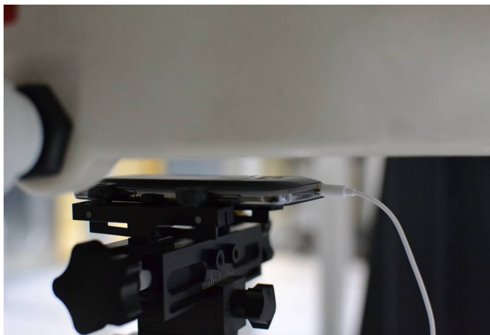
SAR Test Setup Photo 10 – Back side body-worn at 1.0 cm
