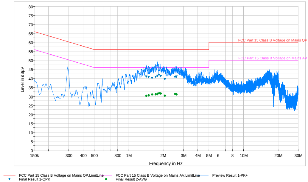
Plot 6-42. Line Conducted Plot with 802.11a UNII Band 2 (N)
