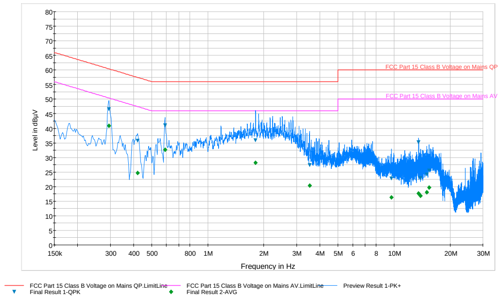
Plot 6-39. Line Conducted Plot with 802.11a UNII Band 1 (L1)
