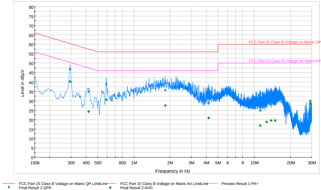
Plot 6-43. Line Conducted Plot with 802.11a UNII Band 3 (L1)
