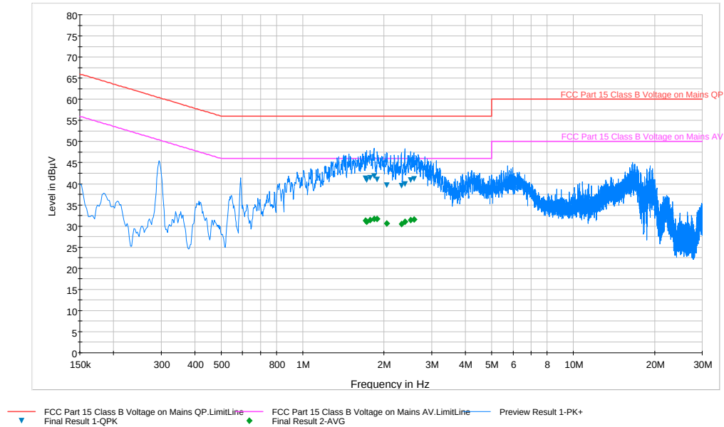
Plot 6-44. Line Conducted Plot with 802.11a UNII Band 3 (N)
