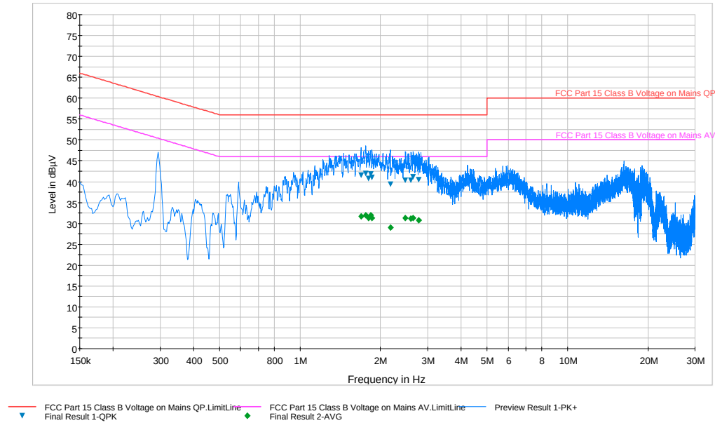
Plot 6-40. Line Conducted Plot with 802.11a UNII Band 1 (N)
