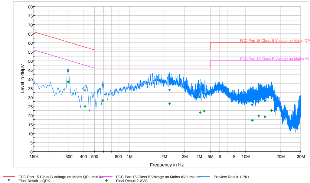
Plot 6-41. Line Conducted Plot with 802.11a UNII Band 2 (L1)
