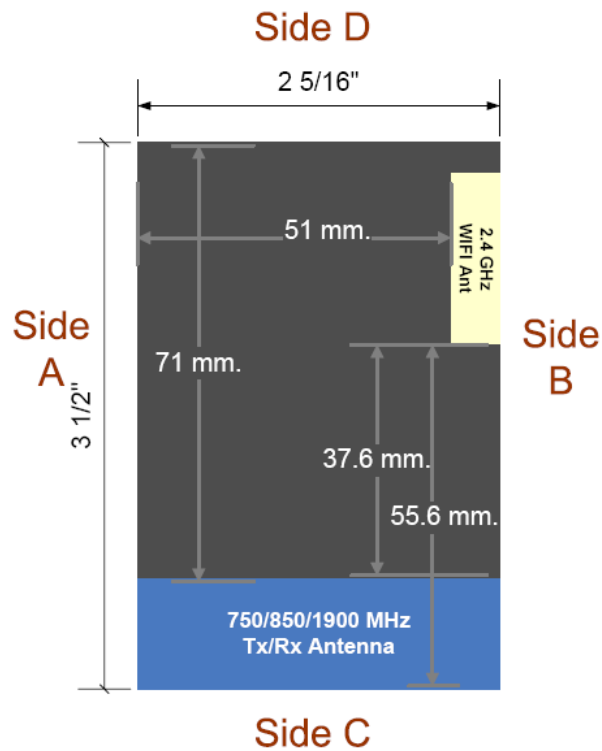
Figure 13-3 Antenna Locations, as viewed from back of device
