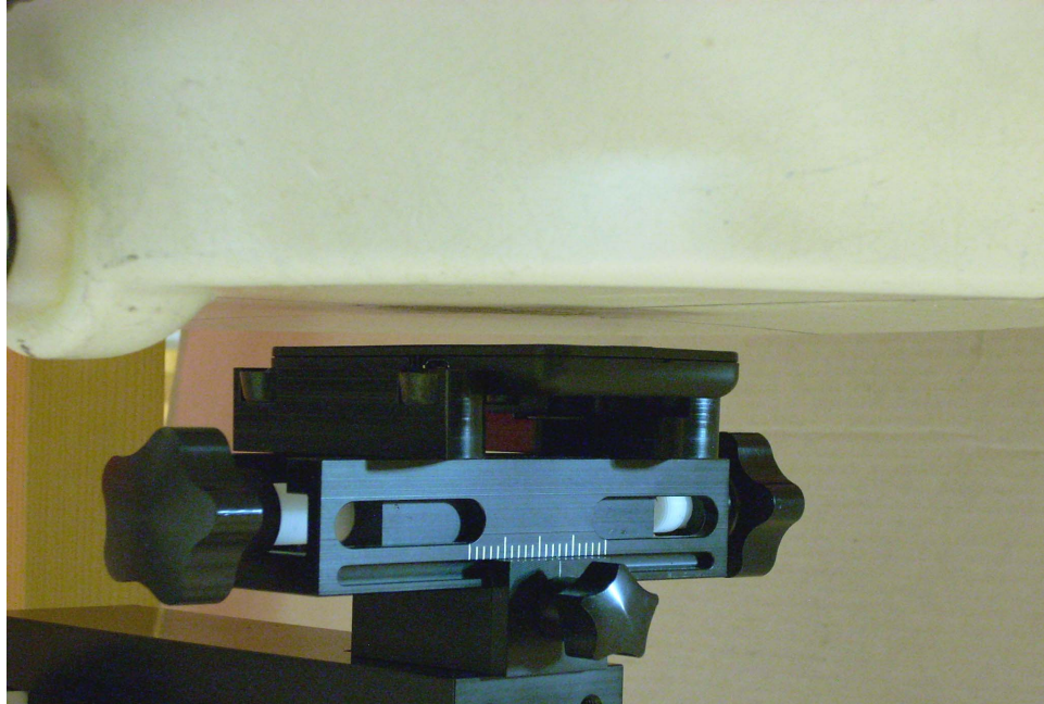
Figure 20-1 SAR Test Setup Photo – Front at 1.0cm
