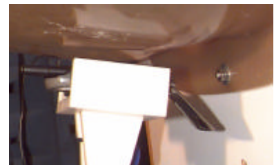
Figure 15. Body SAR Test Setup
