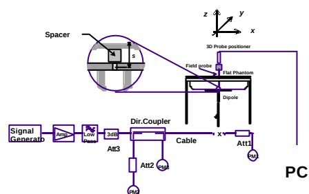
Figure 7.1 Dipole Validation Test Setup
