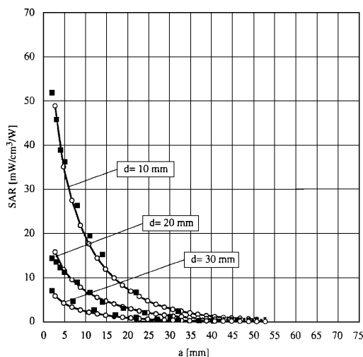
Figure 7. E-Field and temperature measurements at 1.8GHz [6]
