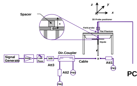
Figure 7.1 Dipole Validation Test Setup
