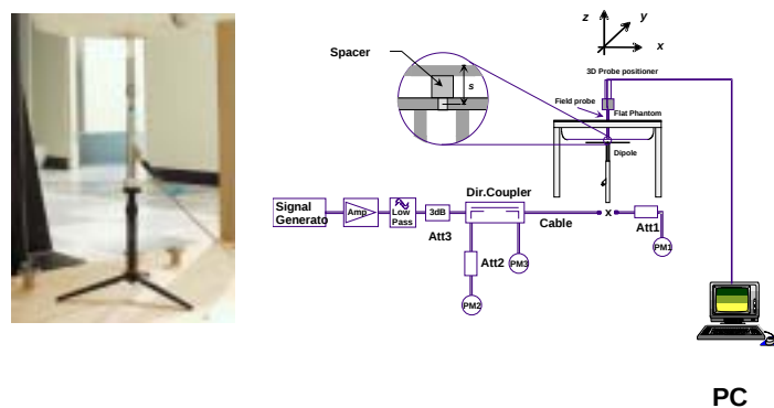
Figure 7.1 Dipole Validation Test Setup
