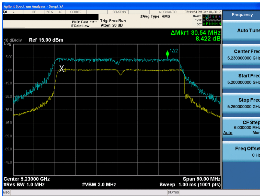
Plot 6-58. Peak Excursion Ratio Plot (40MHz BW 802.11a/n (UNII Band 1) – Ch. 46)
