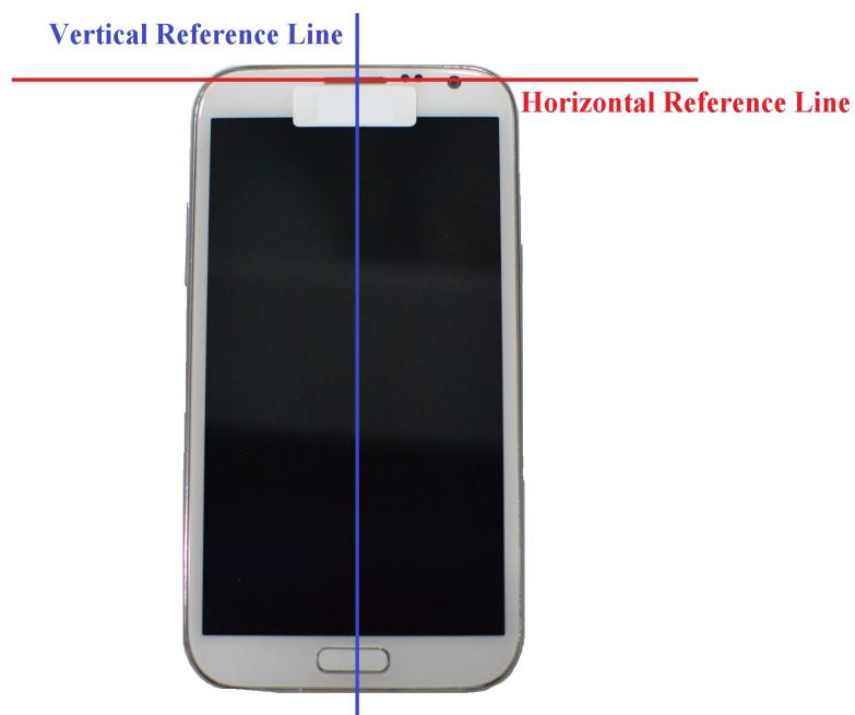
SAR Test Setup Photo 6 – DUT Vertical and Horizontal Reference Lines
