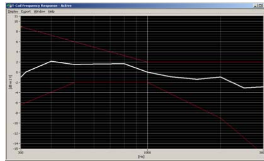
Figure 6-1 Axial Frequency Response
