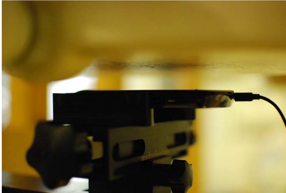
SAR Test Setup Photo 5: Body-Worn Back at 1.5 cm
