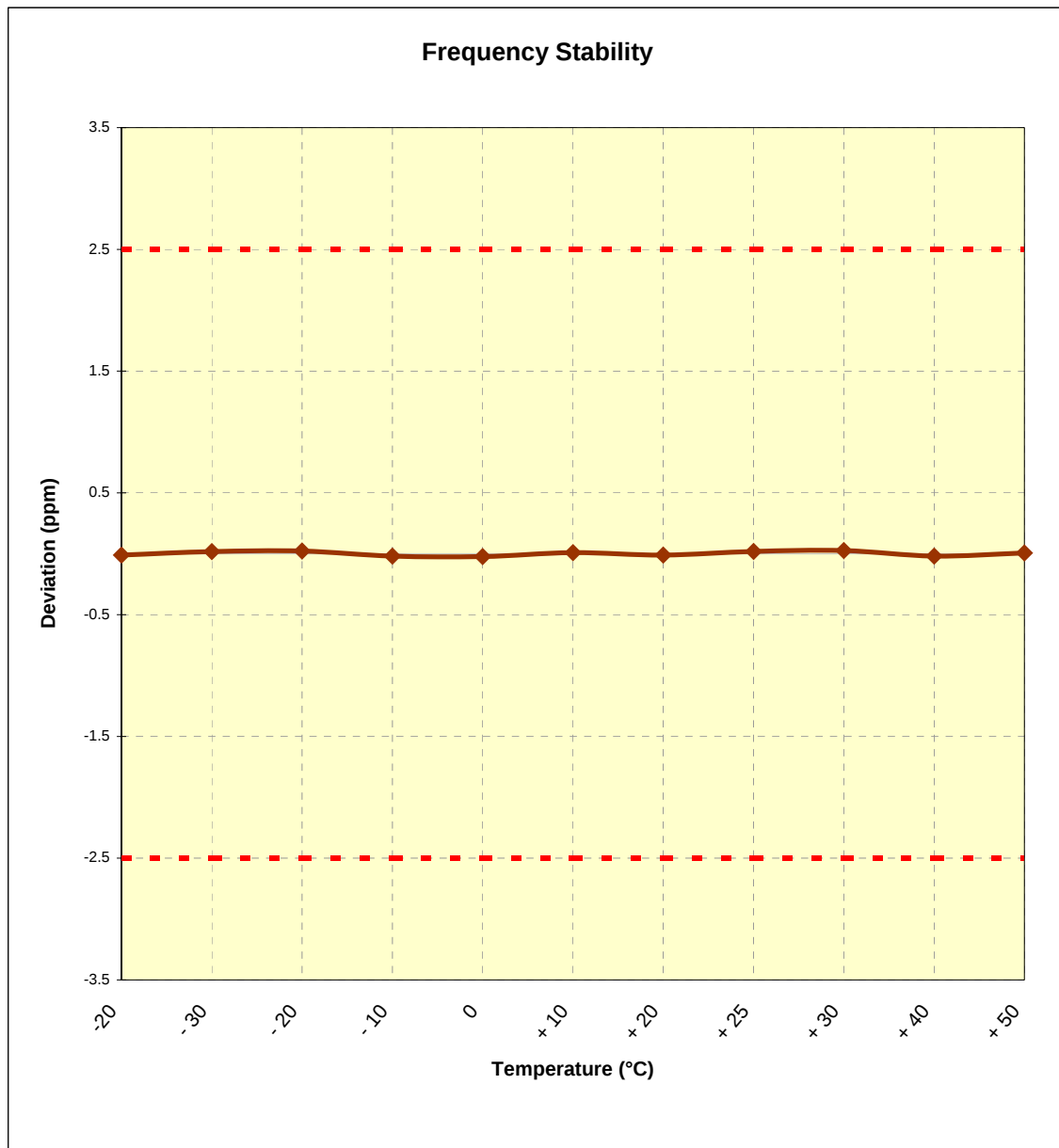
Figure 6-1. Frequency Stability Graph (Cellular CDMA Mode – Ch. 384)
