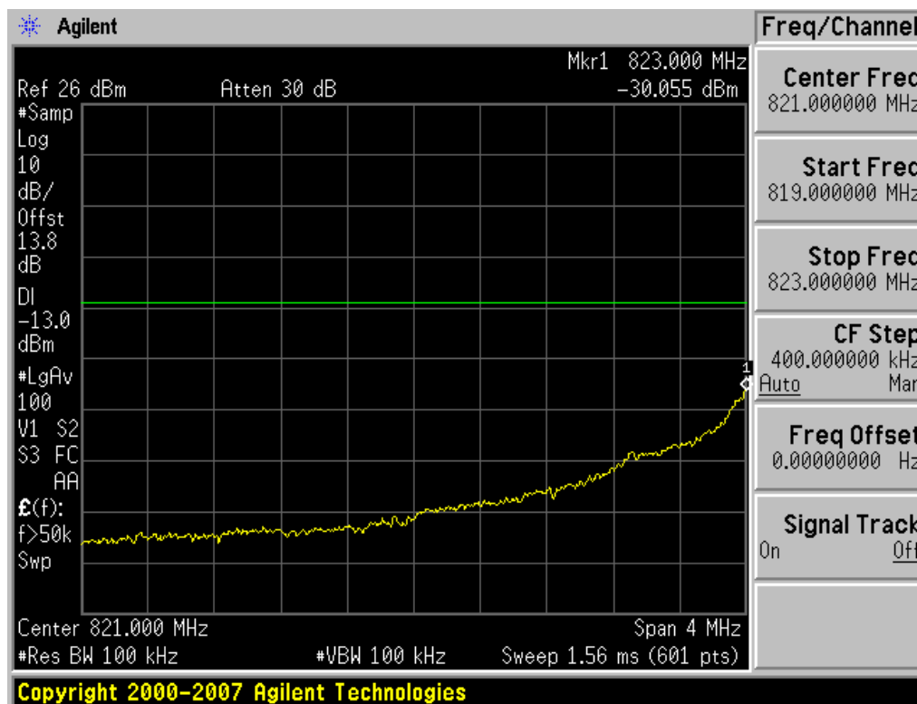
Plot 7-4. 4MHz Span Plot (Cellular CDMA Mode – Ch. 1013)
