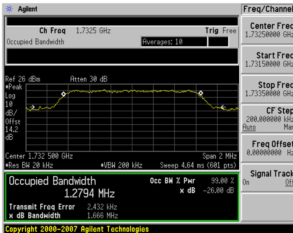
Plot 7-18. Occupied Bandwidth Plot (AWS CDMA Mode – Ch. 450)
