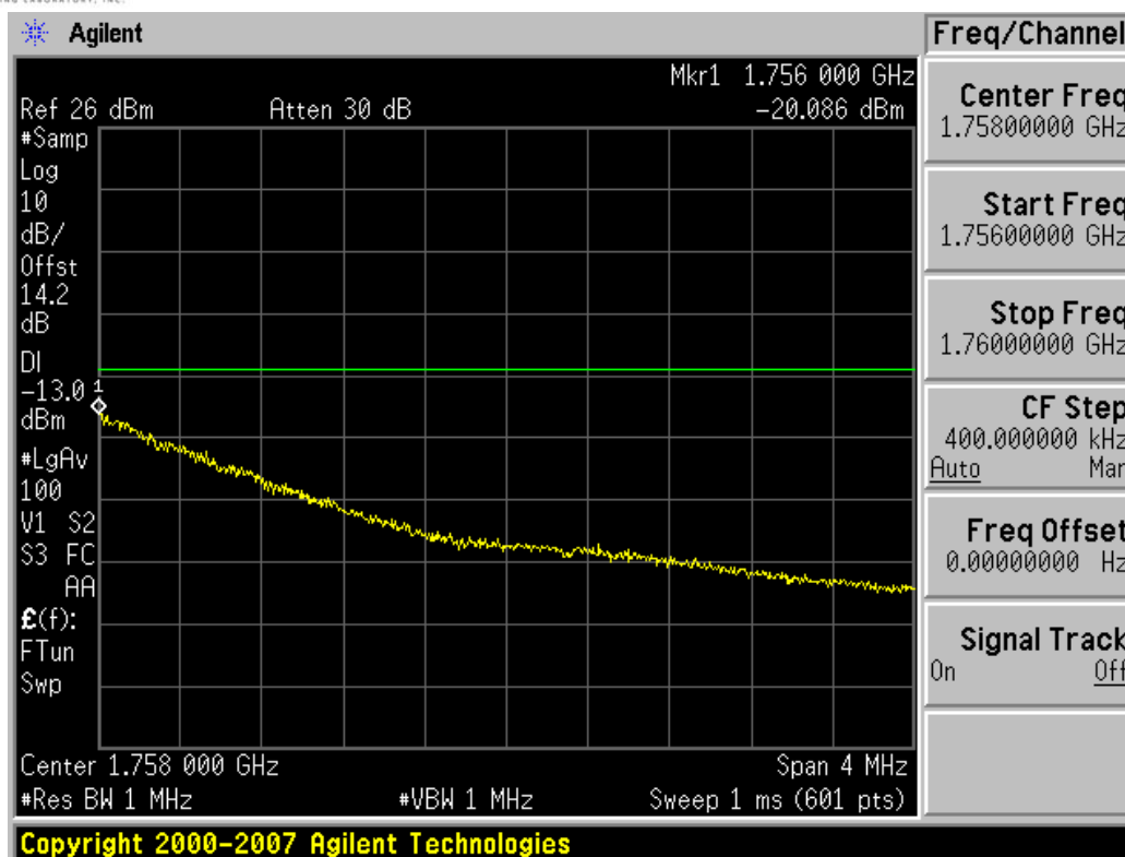
Plot 7-23. 4MHz Span Plot (AWS CDMA Mode – Ch. 875)
