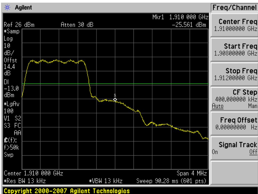
Plot 7-34. Band Edge Plot (PCS CDMA Mode – Ch. 1175)
