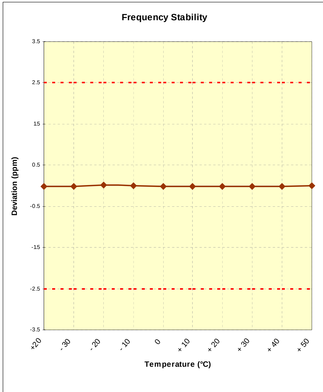
Figure 6-2. Frequency Stability Graph (AWS CDMA Mode – Ch. 450)
