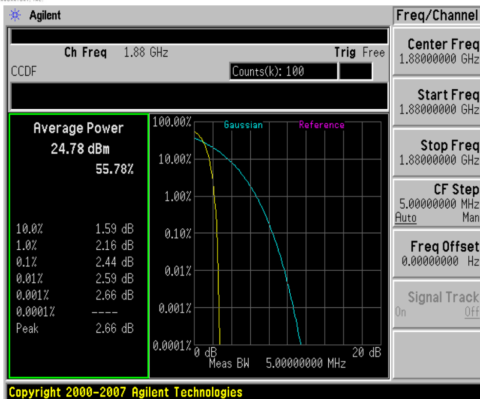
Plot 7-31. Peak-Average Ratio Plot (PCS CDMA Mode – Ch. 600)
