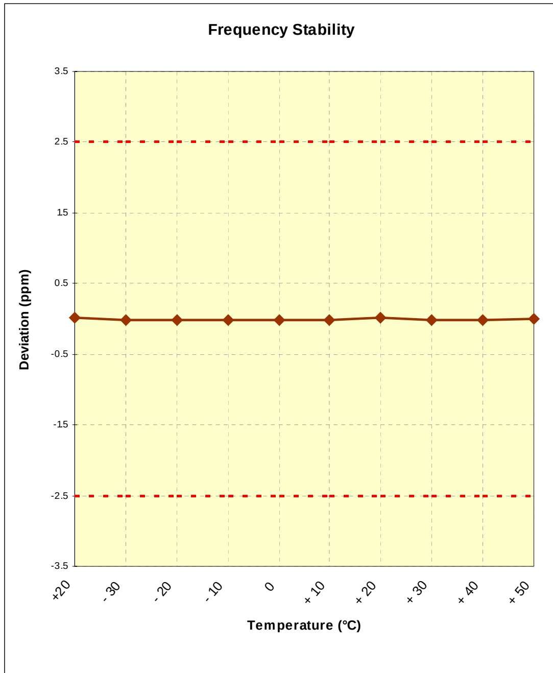
Figure 6-3. Frequency Stability Graph (PCS CDMA Mode – Ch. 600)
