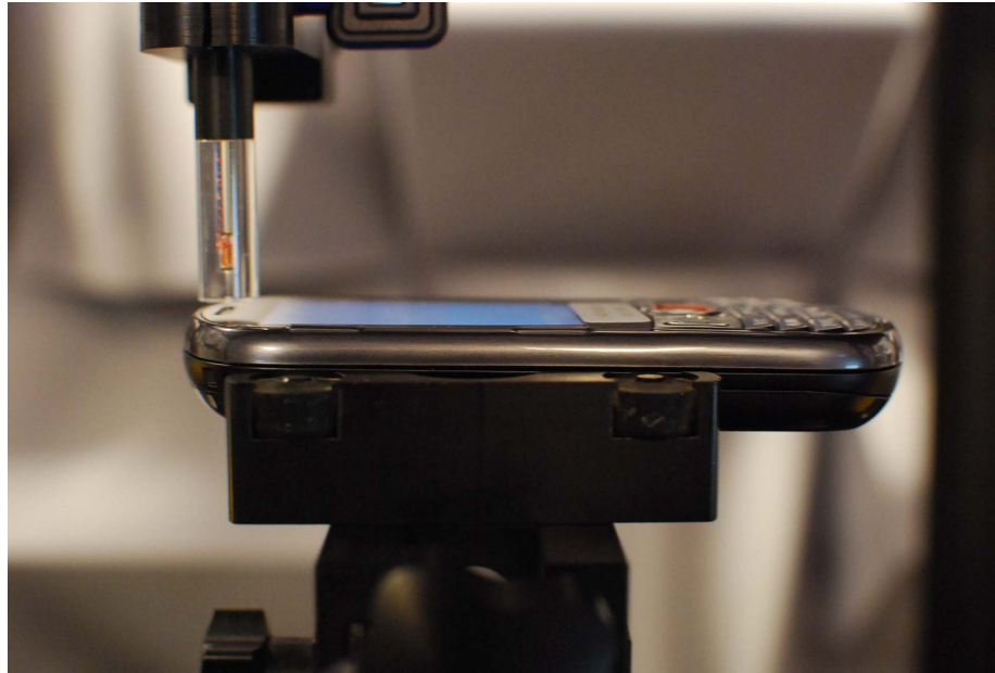
Figure 13-1 Test Setup for Wireless Device
