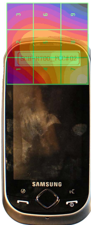
Figure 17-5 H-Field WD Scan overlay
