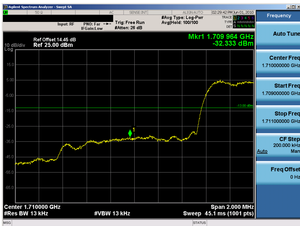
Plot 7-14. Band Edge Plot (AWS CDMA Mode – Ch. 25)
