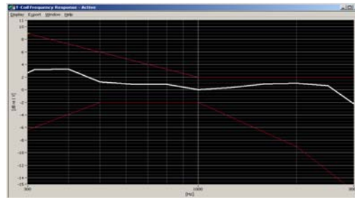
Figure 6-1 Axial Frequency Response
