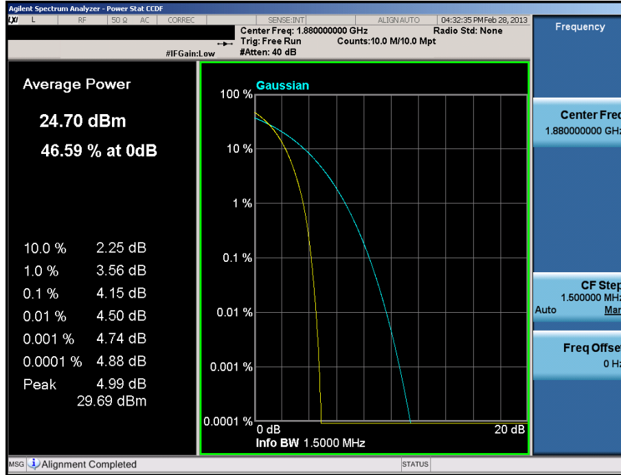
Plot 7-31. Peak-Average Ratio Plot (PCS CDMA Mode – Ch. 600)
