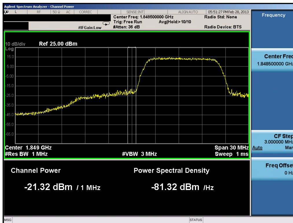
Plot 10-10. Lower Extended Band Edge Plot (10.0MHz QPSK – RB Size 50)
