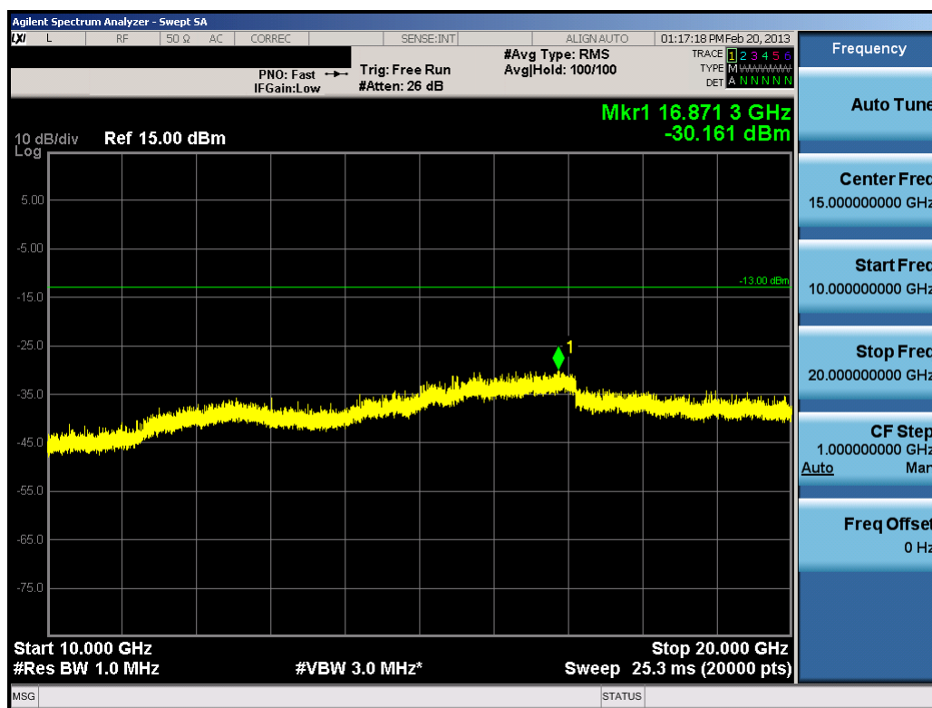
Plot 10-16. Conducted Spurious Plot (10.0MHz QPSK – RB Size 1, RB Offset 0 – Mid Channel)
