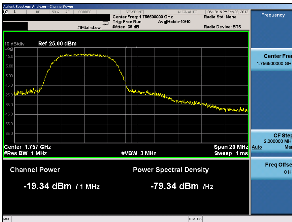
Plot 9-6. Upper Extended Band Edge Plot (5.0MHz QPSK – RB Size 25)
