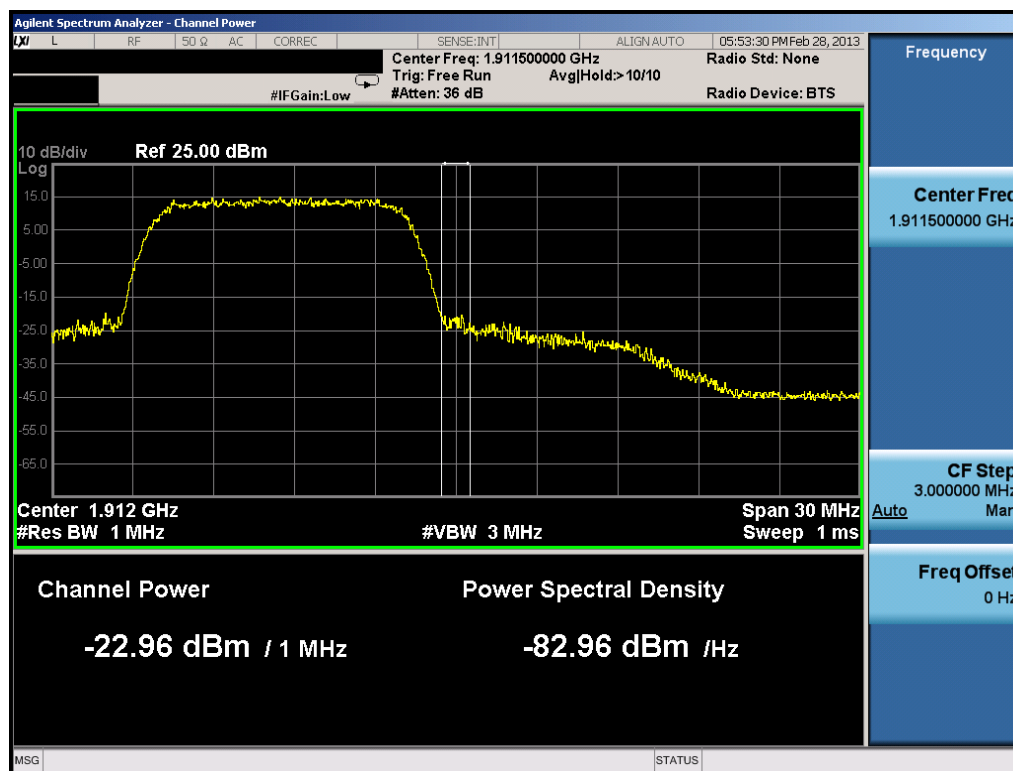
Plot 10-20. Upper Extended Band Edge Plot (10.0MHz QPSK – RB Size 50)
