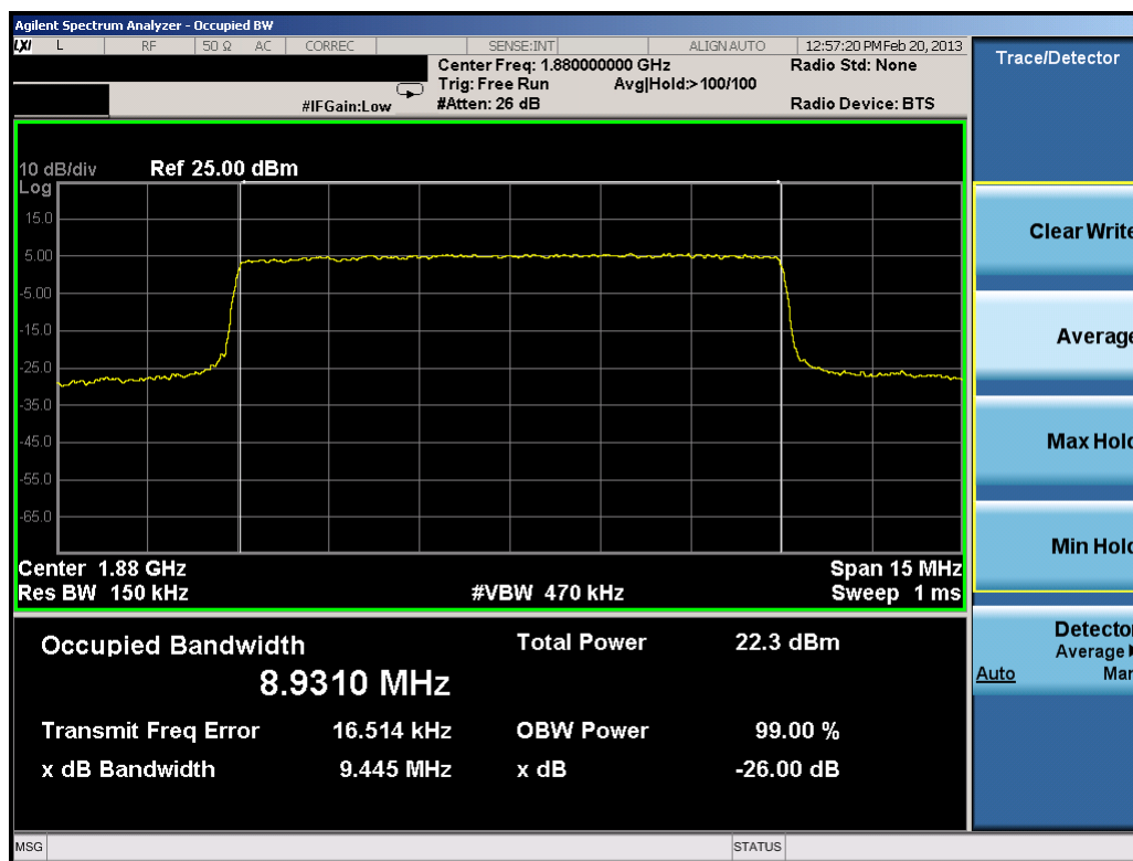
Plot 10-11. Occupied Bandwidth Plot (10.0MHz QPSK – RB Size 50)
