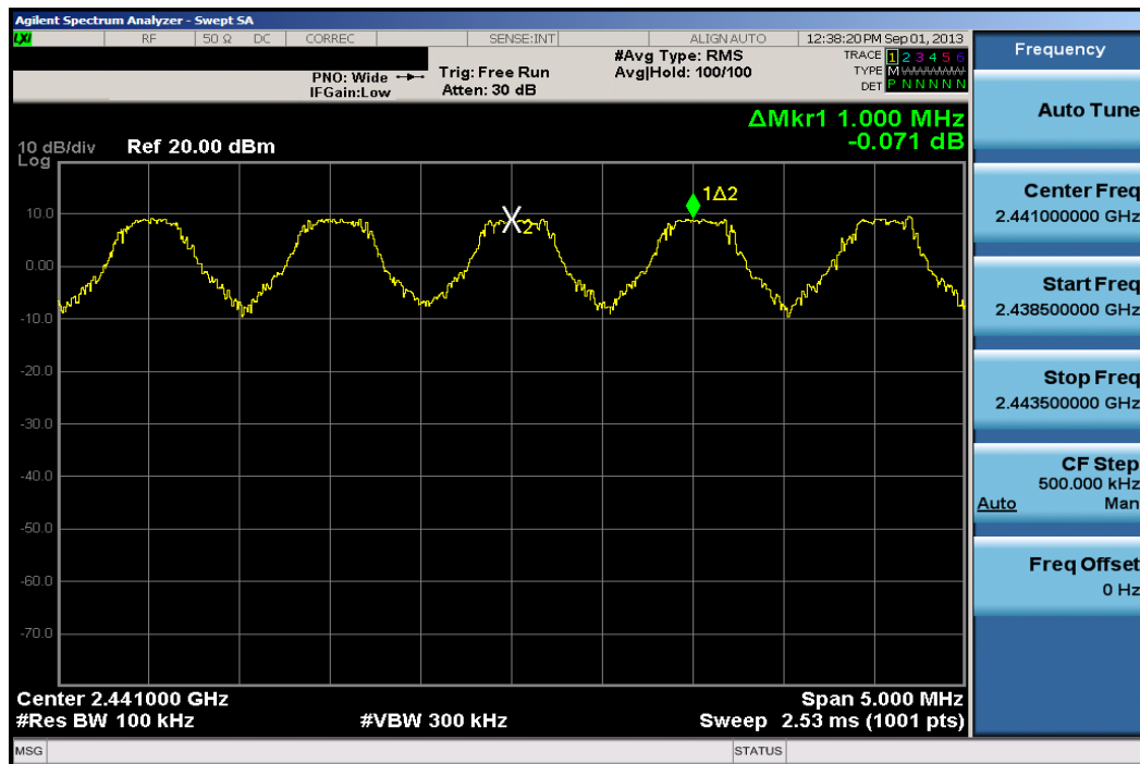
Plot 6-32. Channel Spacing Plot (Bluetooth)
