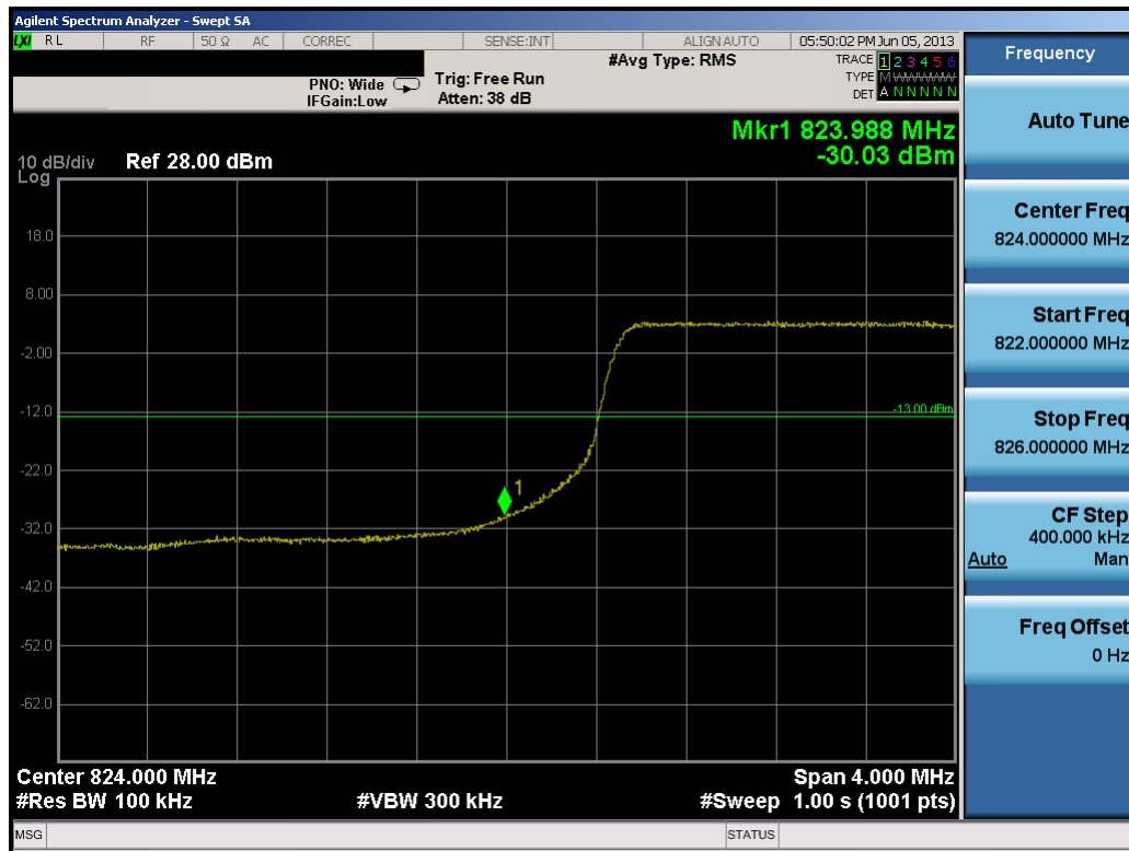
Plot 9-13. Lower Band Edge Plot (10.0MHz QPSK – RB Size 50)
