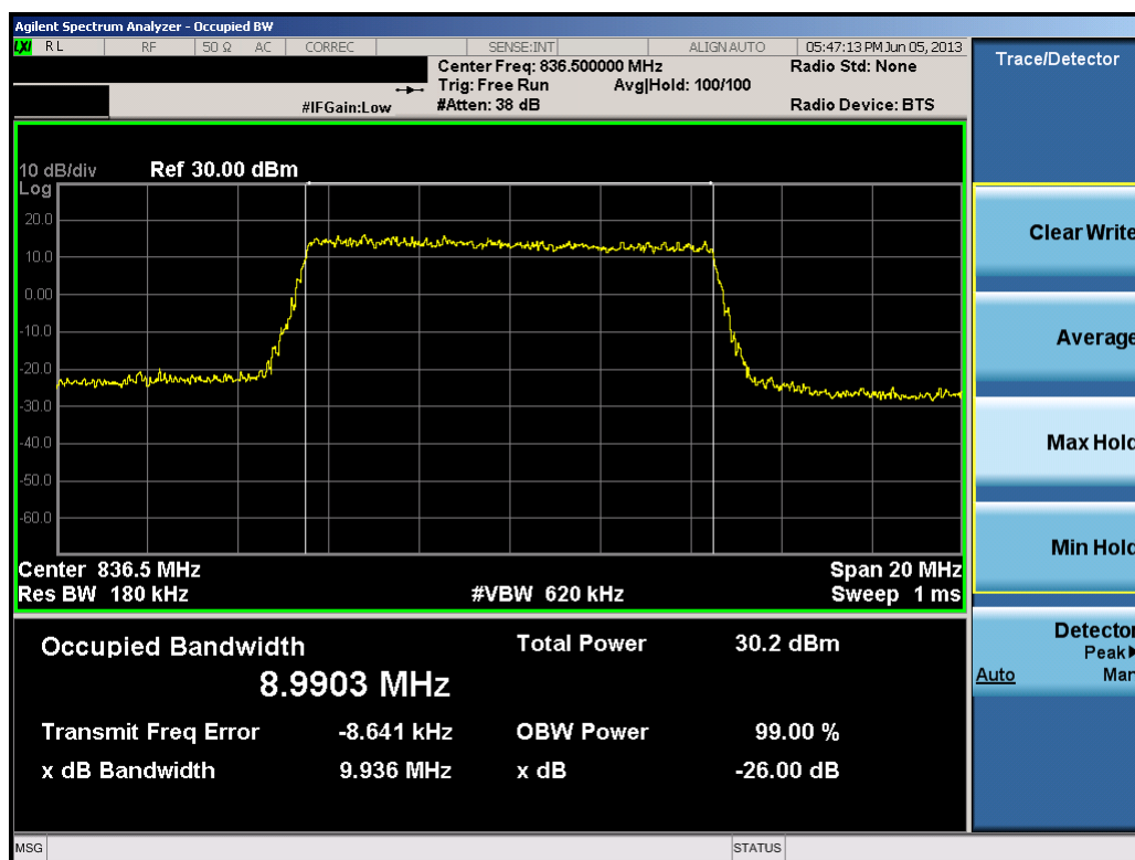
Plot 9-15. Occupied Bandwidth Plot (10.0MHz QPSK – RB Size 50)
