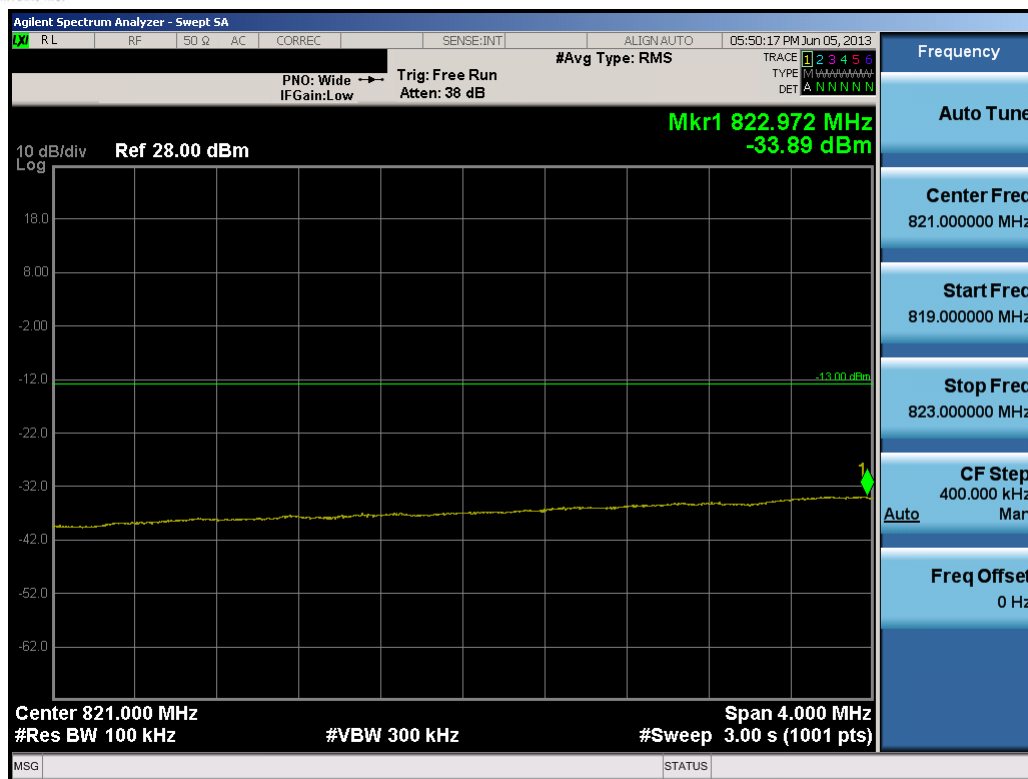
Plot 9-14. Lower Extended Band Edge Plot (10.0MHz QPSK – RB Size 50)
