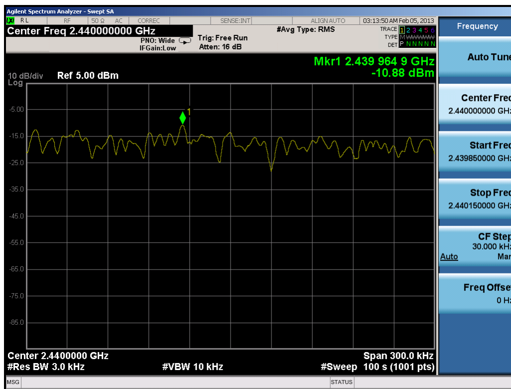
Plot 6-5. Power Spectral Density Plot (Bluetooth (LE) – Ch. 19)
