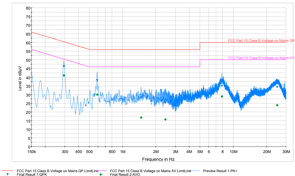
Plot 6-19. Line Conducted Plot with Bluetooth LE (L1)
