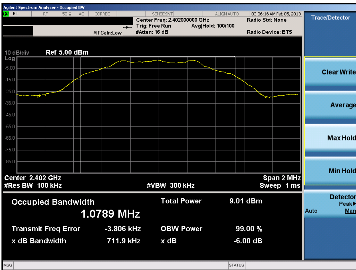
Plot 6-1. 6dB Bandwidth Plot (Bluetooth (LE) - Ch. 0)
