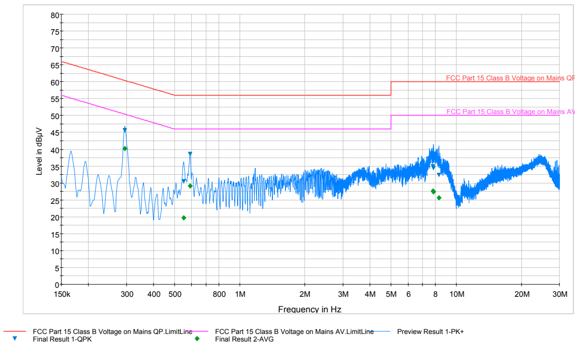
Plot 6-20. Line Conducted Plot with Bluetooth LE (N)
