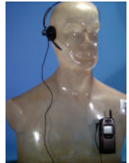
Figure 7. Ear-Microphone Jack
