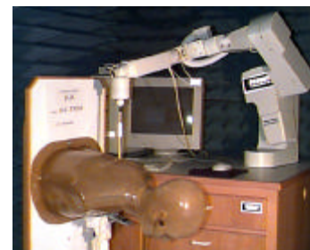
Fig. 1 SAR Test Setup
