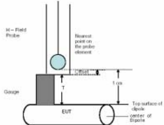
Figure 5.3 Gauge block with H-field probe
