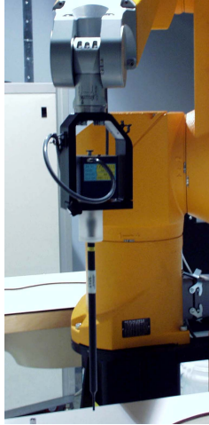
Figure 3.2 DAE System
