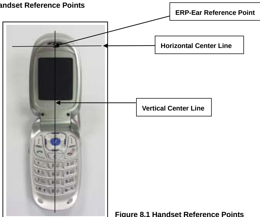
Figure 8.1 Handset Reference Points
