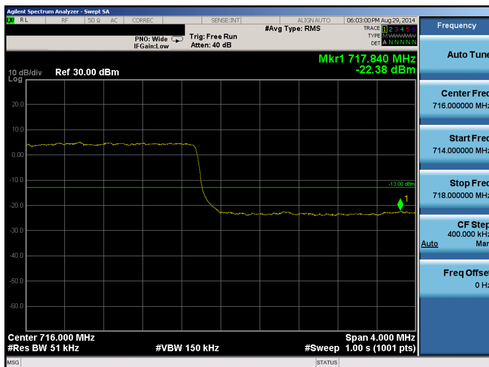
Plot 6-18. Upper Band Edge Plot (Band 17 – 5.0MHz QPSK – RB Size 25)
