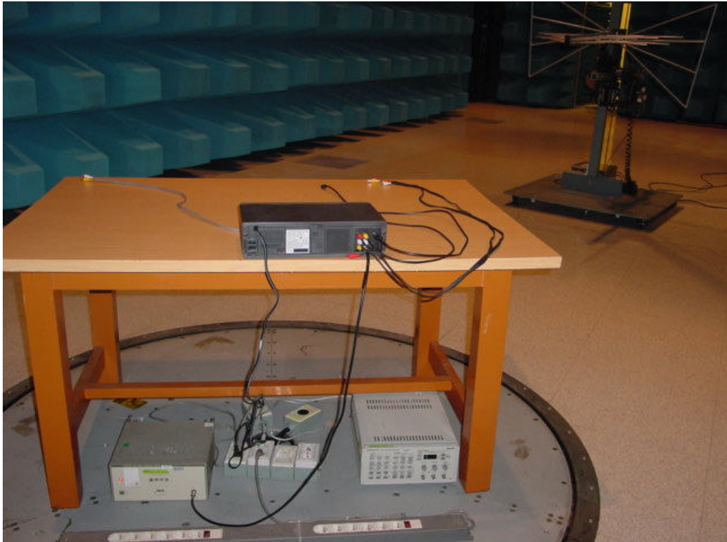
Fig. 2 Test Setup for Radiated Emissions Measurement
