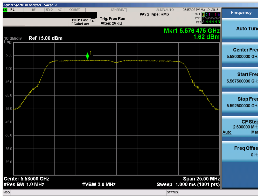
Plot 6-96. Power Spectral Density Plot (802.11a (UNII Band 2C) – Ch. 116)
