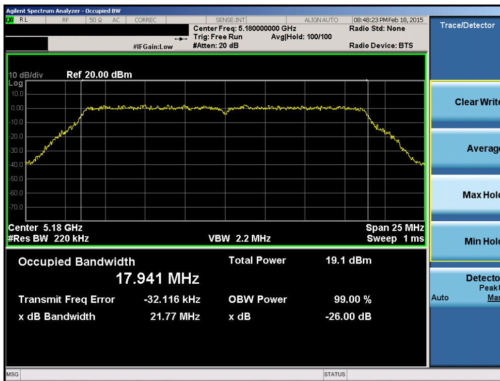
Plot 6-33. 26dB Bandwidth Plot (20MHz BW 802.11n (UNII Band 1) – Ch. 36)
