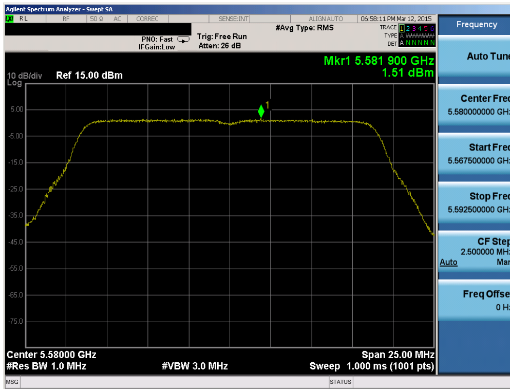
Plot 6-99. Power Spectral Density Plot (20MHz BW 802.11n (UNII Band 2C) – Ch. 116)
