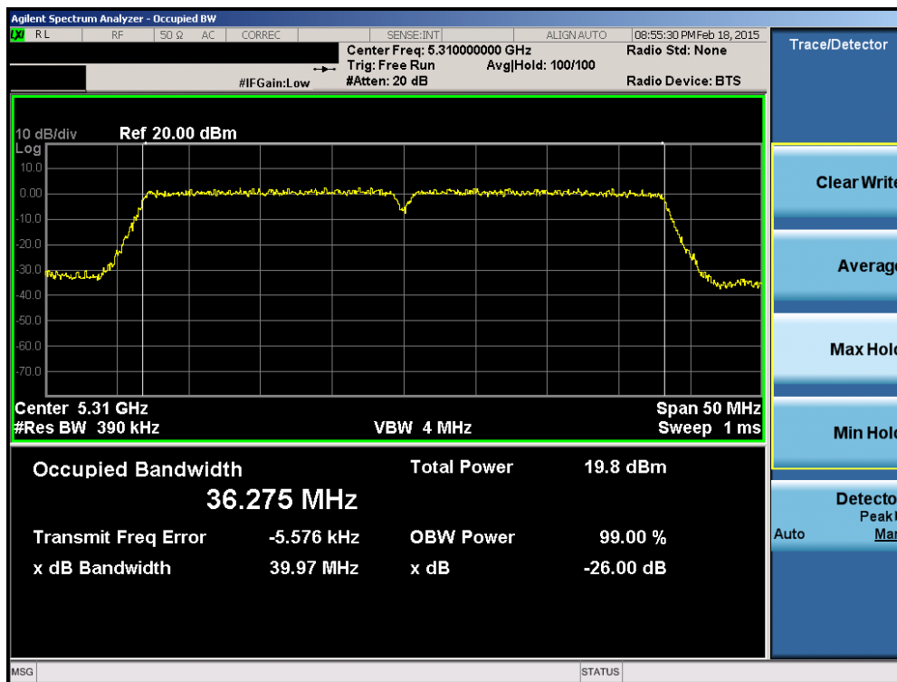
Plot 6-46. 26dB Bandwidth Plot (40MHz BW 802.11n (UNII Band 2A) – Ch. 62)
