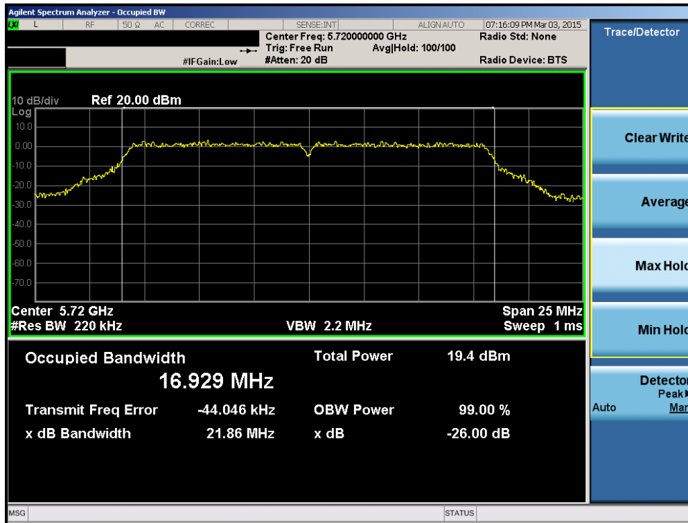
Plot 6-50. 26dB Bandwidth Plot (802.11a (UNII Band 2C) – Ch. 144)
