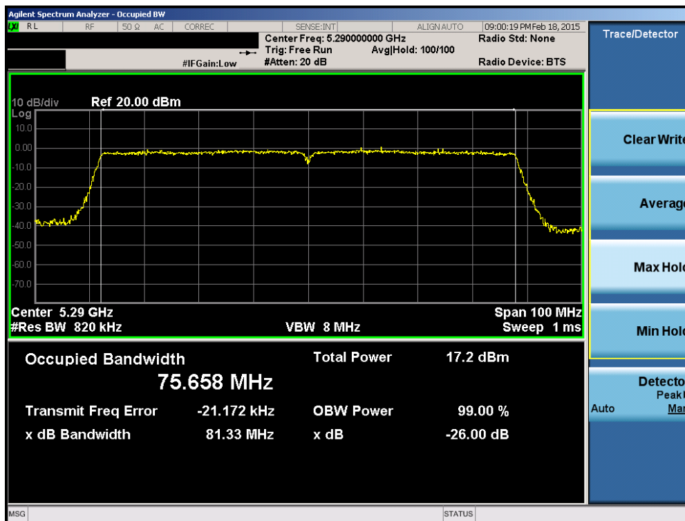
Plot 6-47. 26dB Bandwidth Plot (80MHz BW 802.11ac (UNII Band 2A) – Ch. 58)
