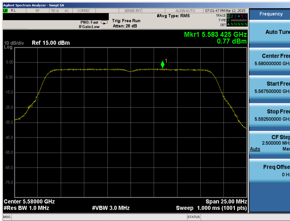
Plot 6-137. Power Spectral Density Plot (20MHz BW 802.11n (UNII Band 2C) – Ch. 116)
