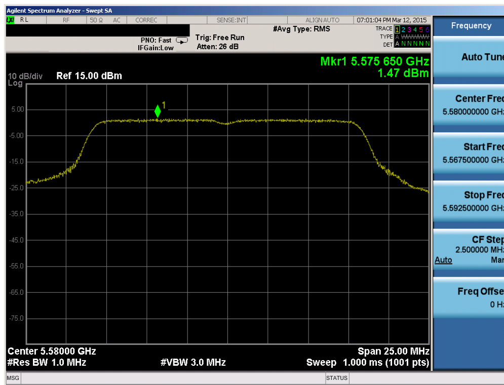
Plot 6-134. Power Spectral Density Plot (802.11a (UNII Band 2C) – Ch. 116)
