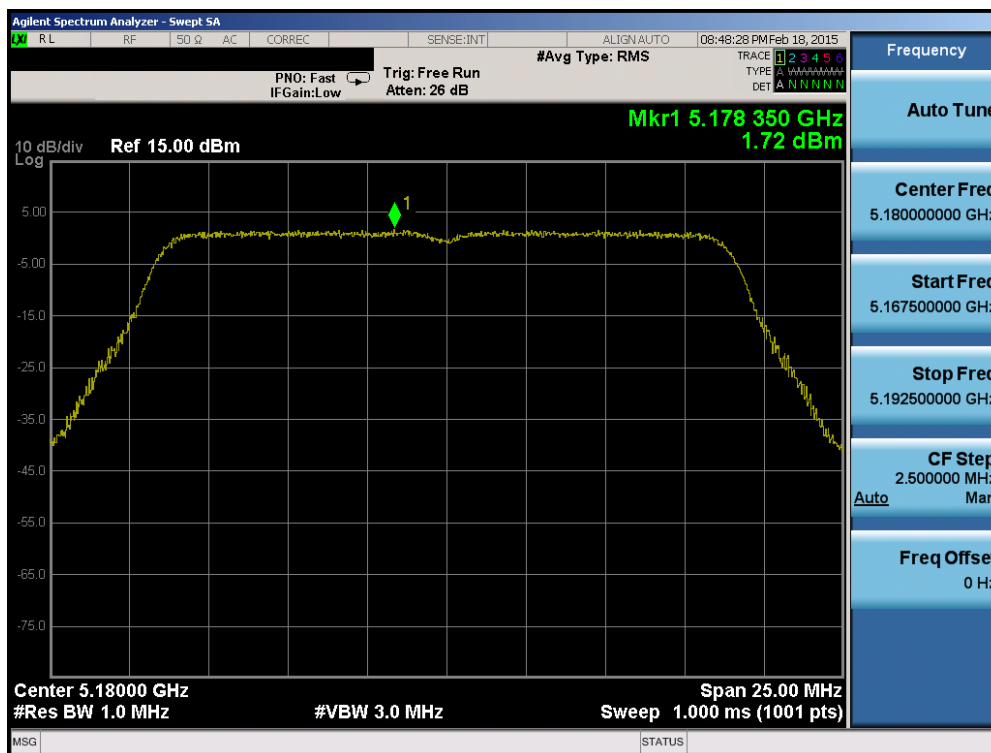
Plot 6-118. Power Spectral Density Plot (20MHz BW 802.11n (UNII Band 1) – Ch. 36)
