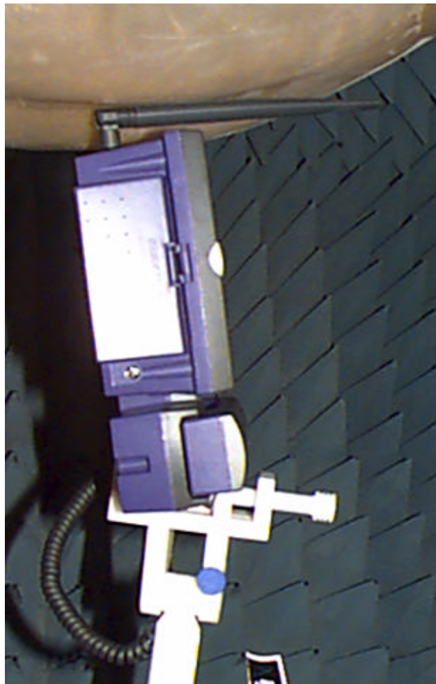
Figure 8. Test setup of EUT in normal operating position with the source of significant emissions (antenna) in direct contact with the phantom.
