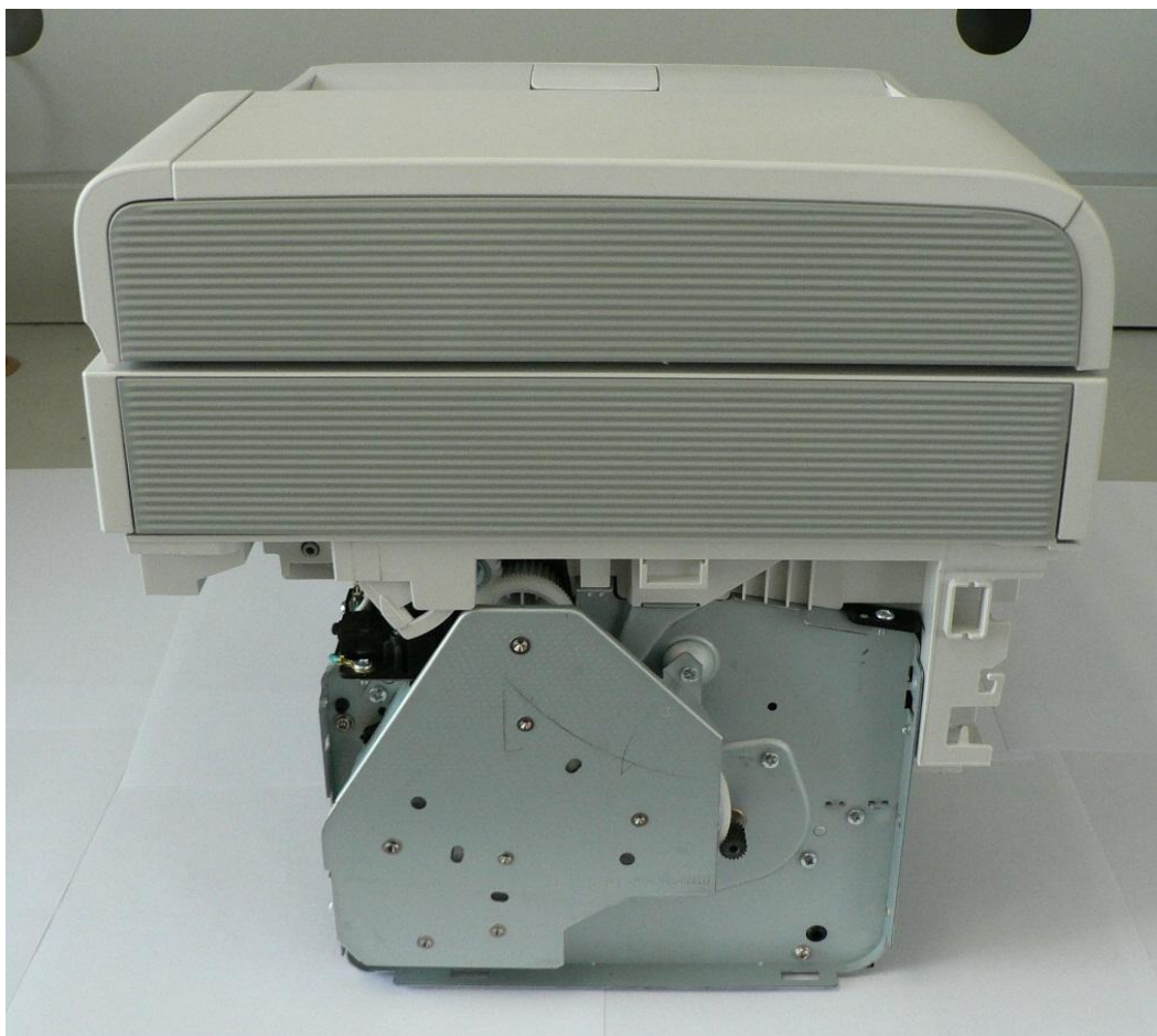
SCX-3405FW SIDE_RIGHT
