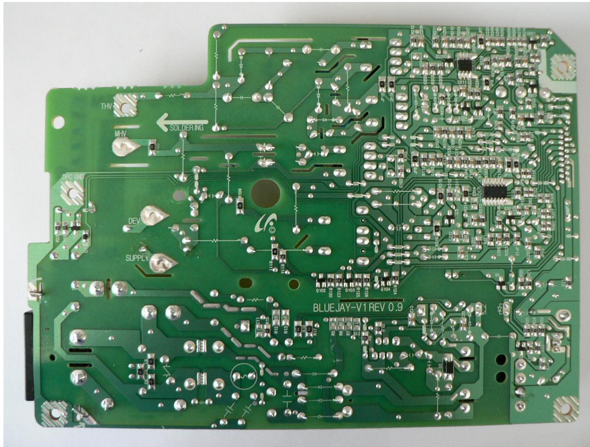
SHANDONG, Bluejay V1 SCX-3405FW SMPS & HVPS PBA_Rear
