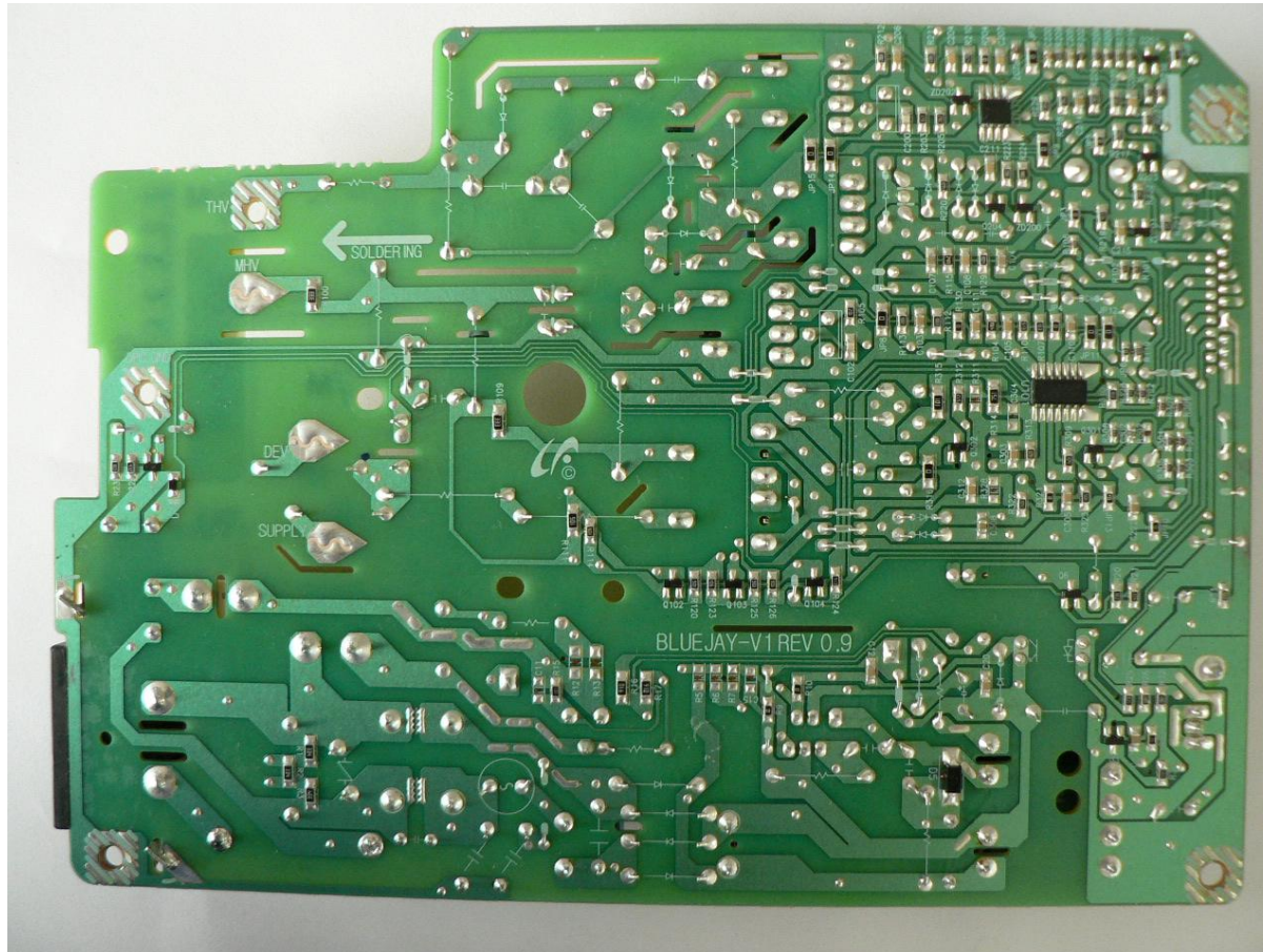
SUNGHO, Bluejay V1 SCX-3405FW SMPS & HVPS PBA_Rear
