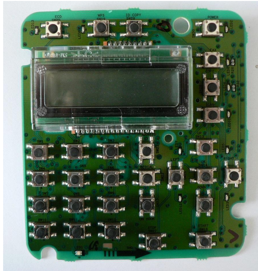
SCX-3405FW OPE PBA_Front
