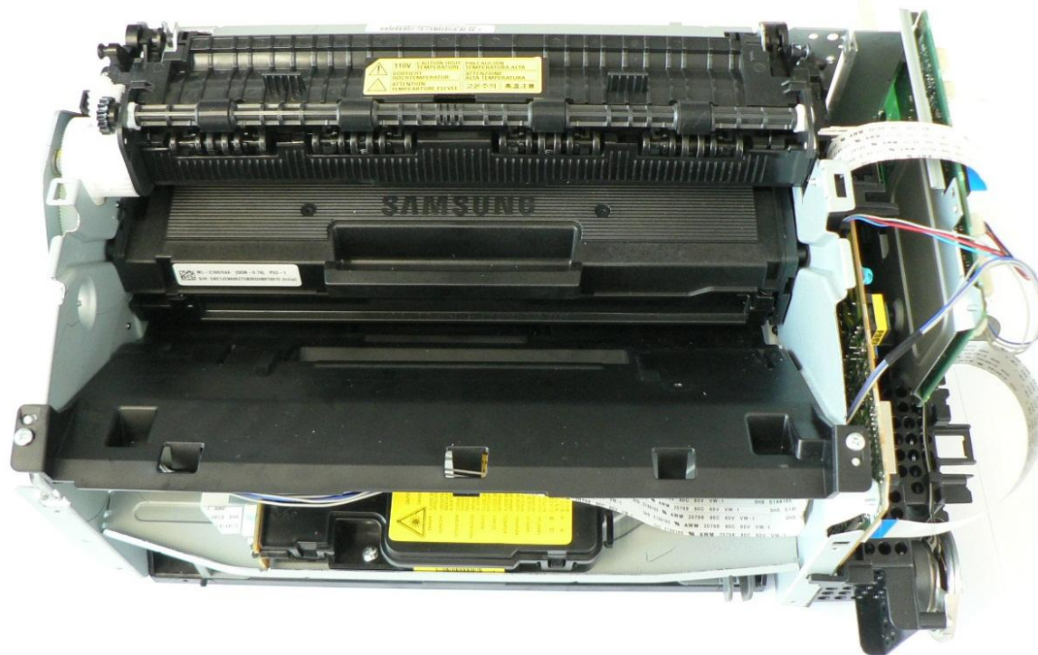
SCX-3405FW TOP VIEW
