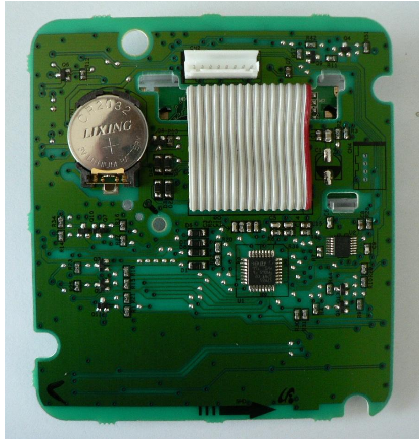
SCX-3405FW OPE PBA_Rear
