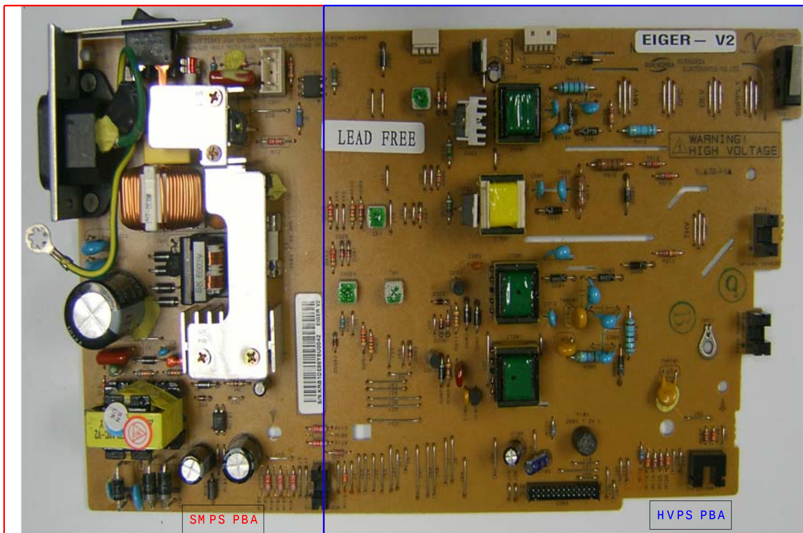
SCX-4200 SMPS/HVPS PBA_Front
