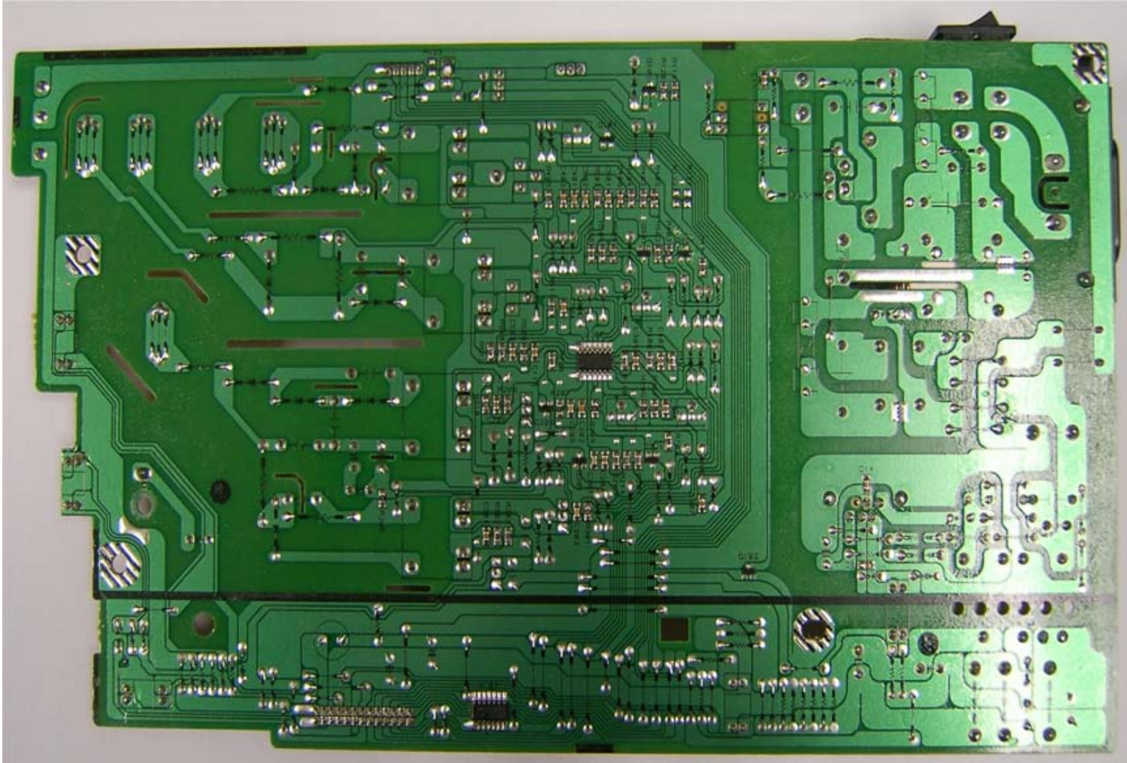
SCX-4200 SMPS/HVPS PBA_Rear
