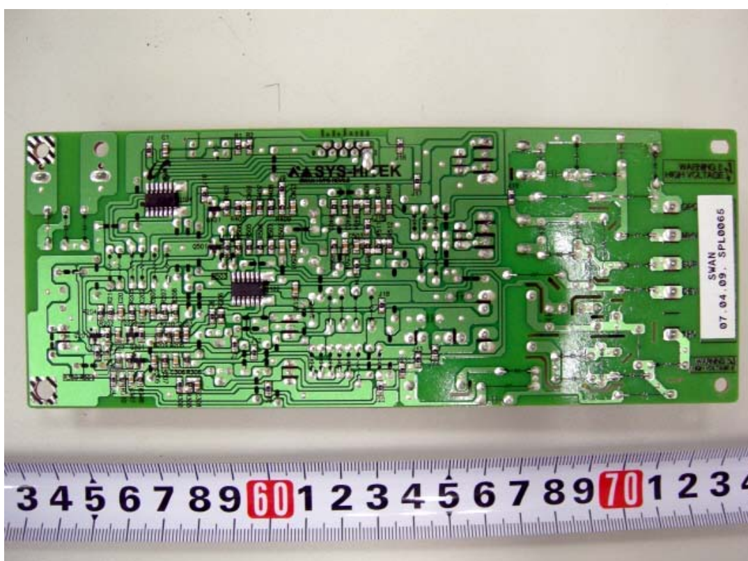
Fig 20 (SCX-4500***, ML-163****)
