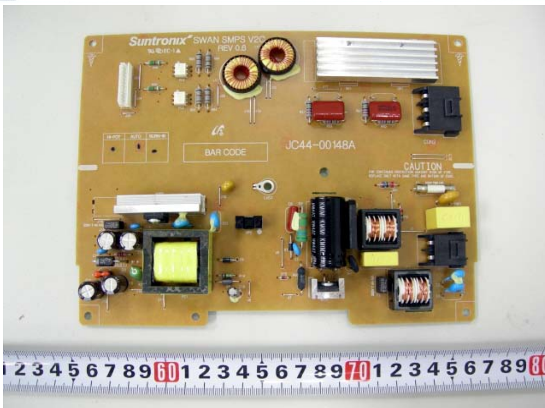
Fig 15 (SCX-4500***, ML-163****)
