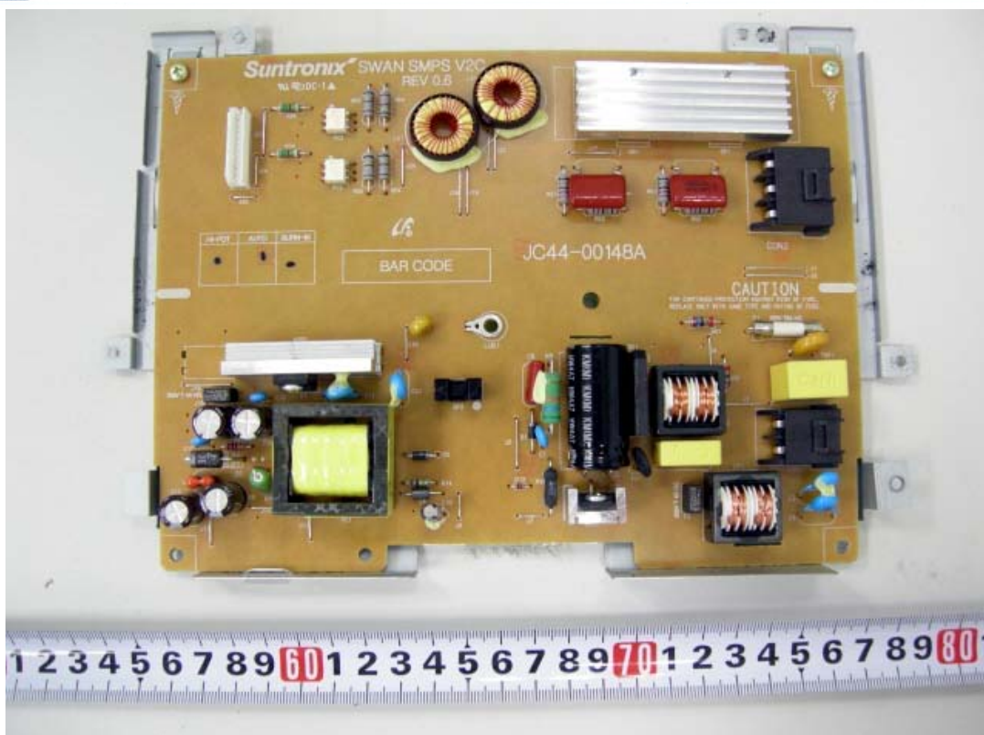
Fig 17 (SCX-4500***, ML-163****)
