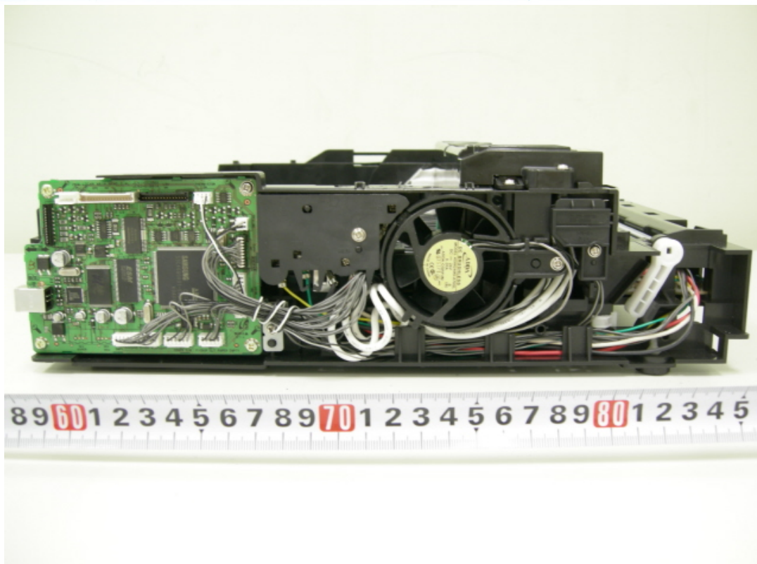
Fig 13 (SCX-450***, ML-163****)
