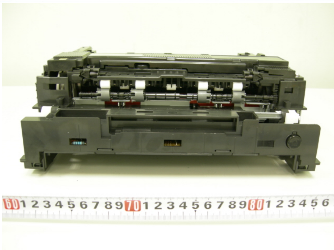
Fig 11 (SCX-4500***, ML-163****)
