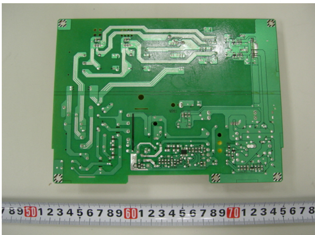
Fig 16 (SCX-4500***, ML-163****)
