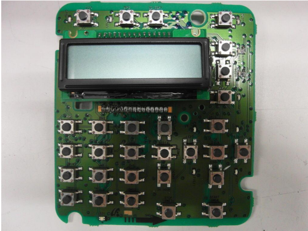
PBA Photo_OPE KEY Front
