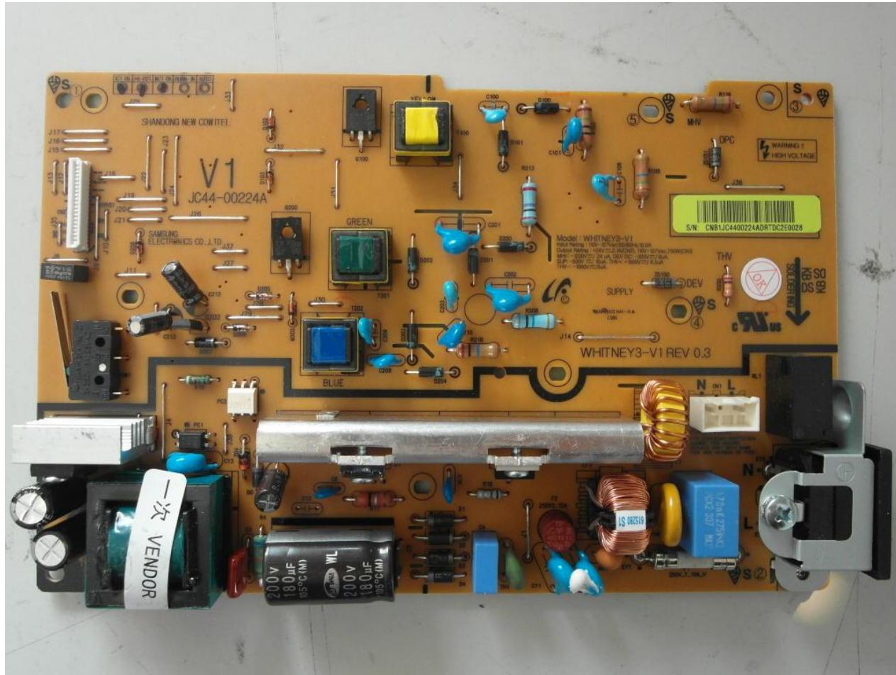
PBA Photo_SMPS+HVPS PBA Front (New Cowitel)
