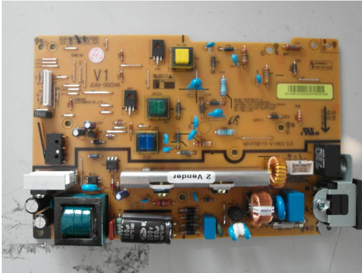
PBA Photo_SMPS+HVPS PBA Front (SUNG HO)
