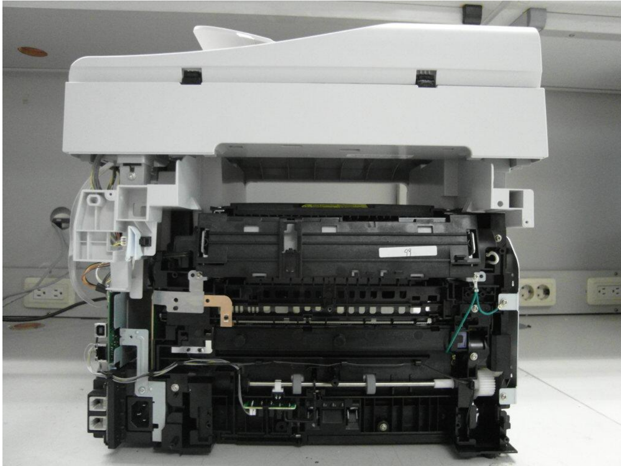
Internal View Photo_Back
