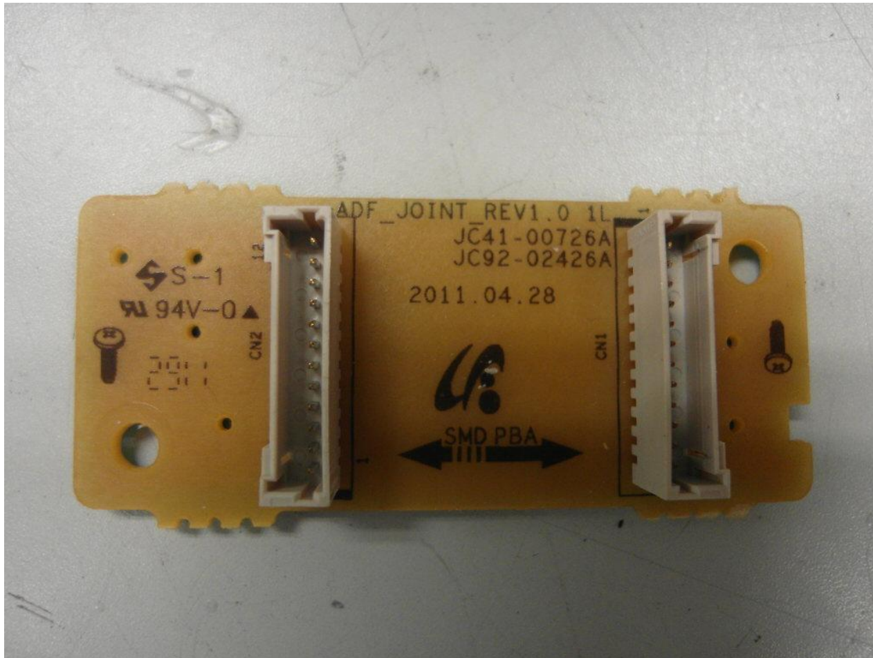
PBA Photo_ADF JOINT PBA Front
