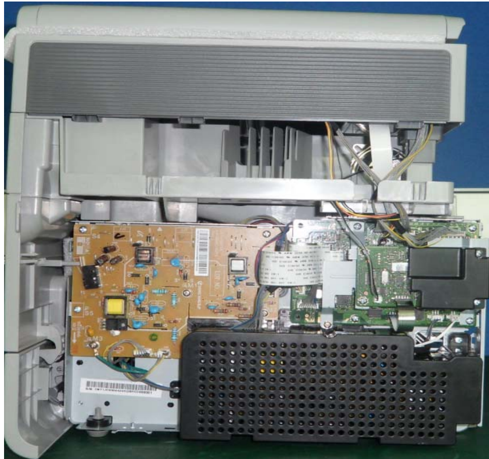
Internal View Photo_Right
