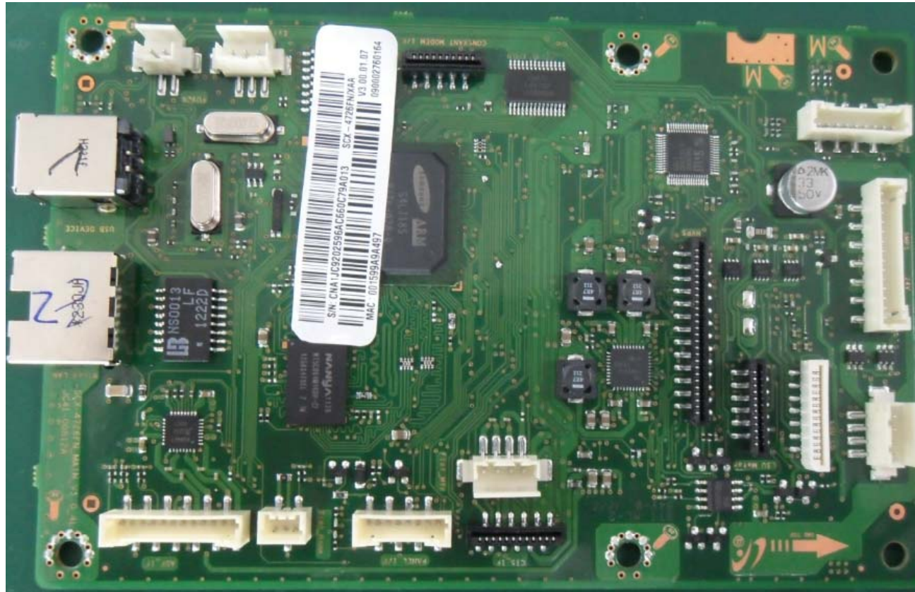
PBA Photo_Main PBA Top
