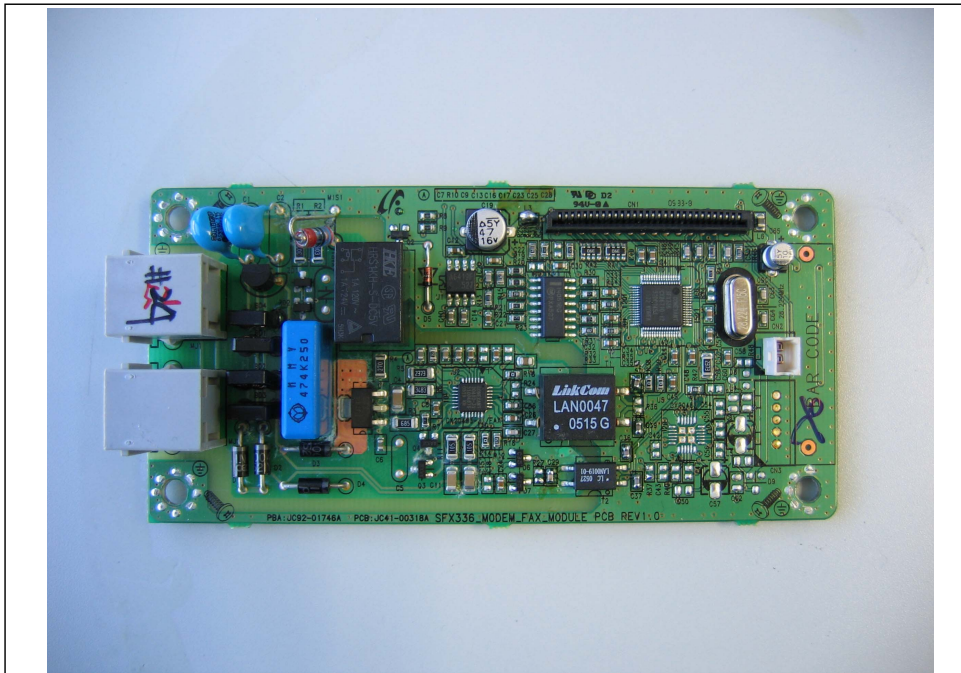
9) Top View of Modem B'd
