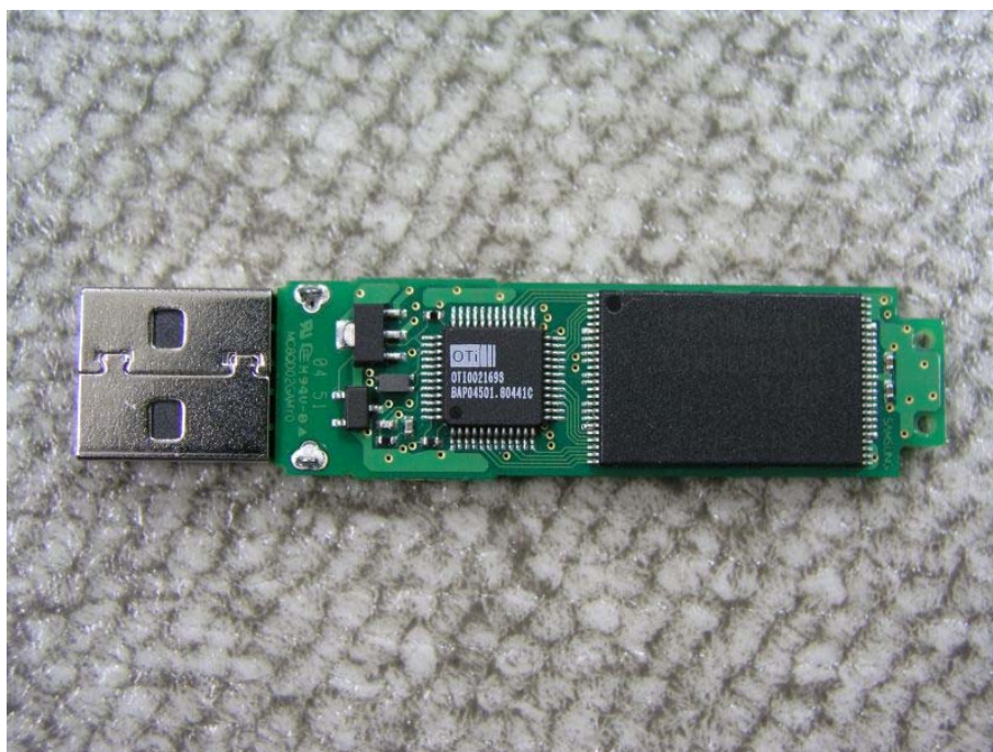
Picture 7. EUT (Internal Front)
