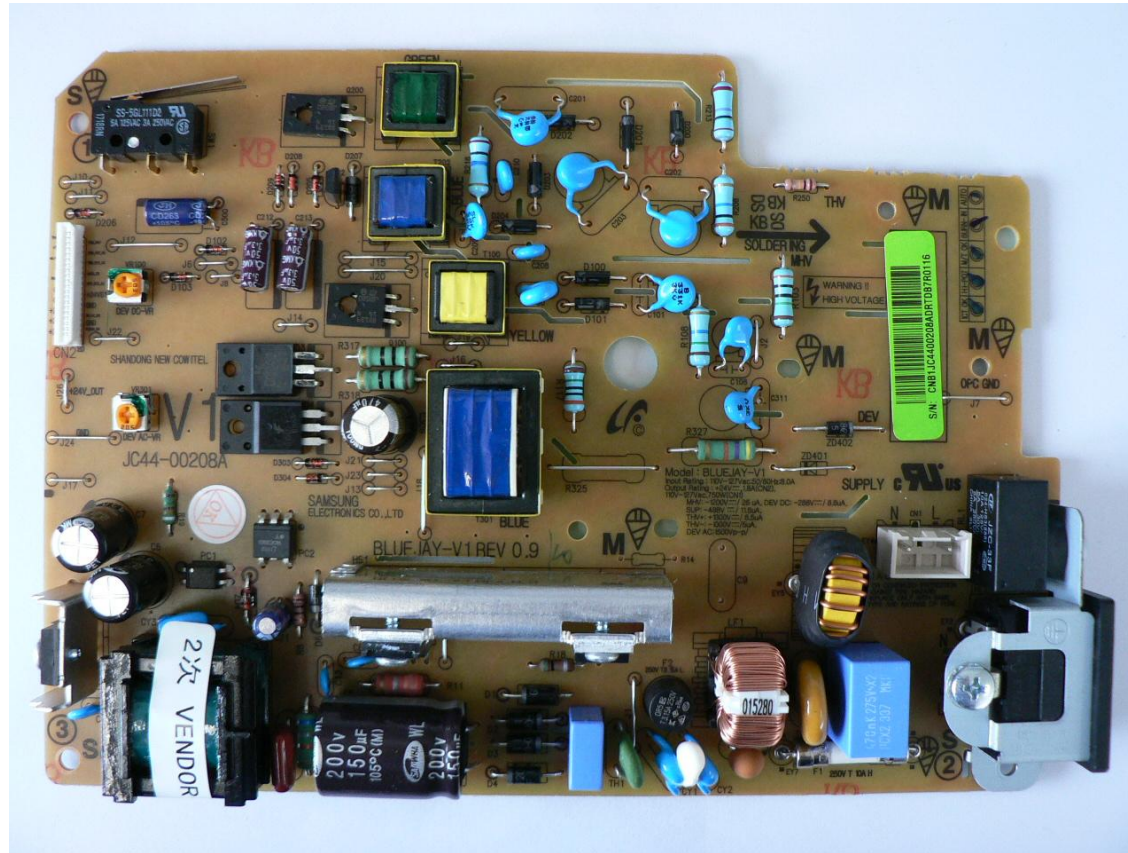
SHANDONG, Bluejay V1 SF-760P SMPS & HVPS PBA_Front
