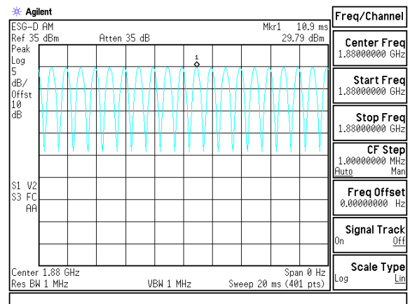
Figure 8-7 PCS 80% AM Signal
