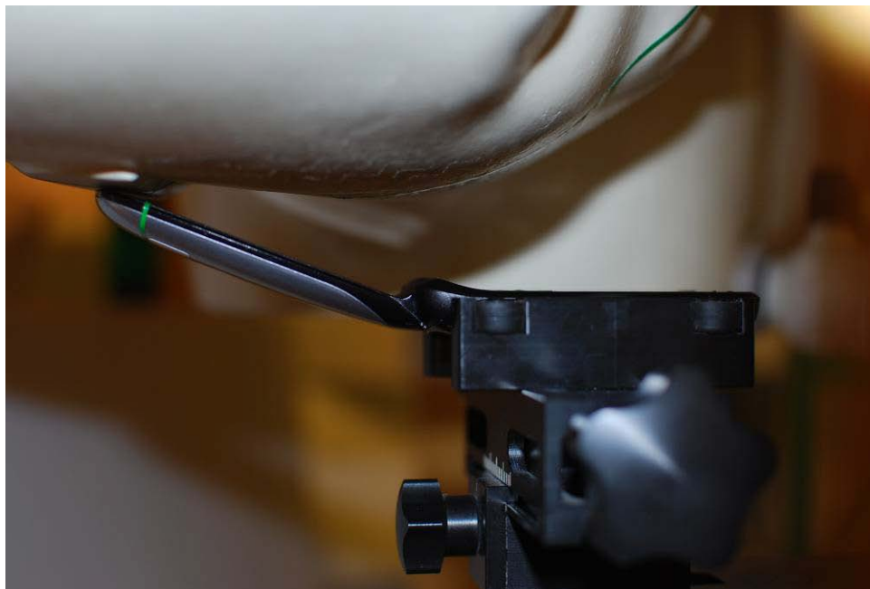
Figure 18-2 SAR Test Setup Photo 2
