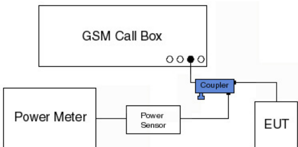
Figure 6-1. GSM Conducted Power Test Setup Diagram
