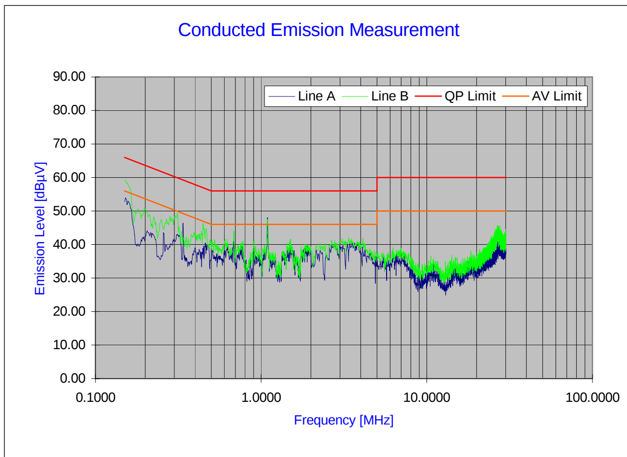
Plot 8-1. Line-Conducted Test Plot
