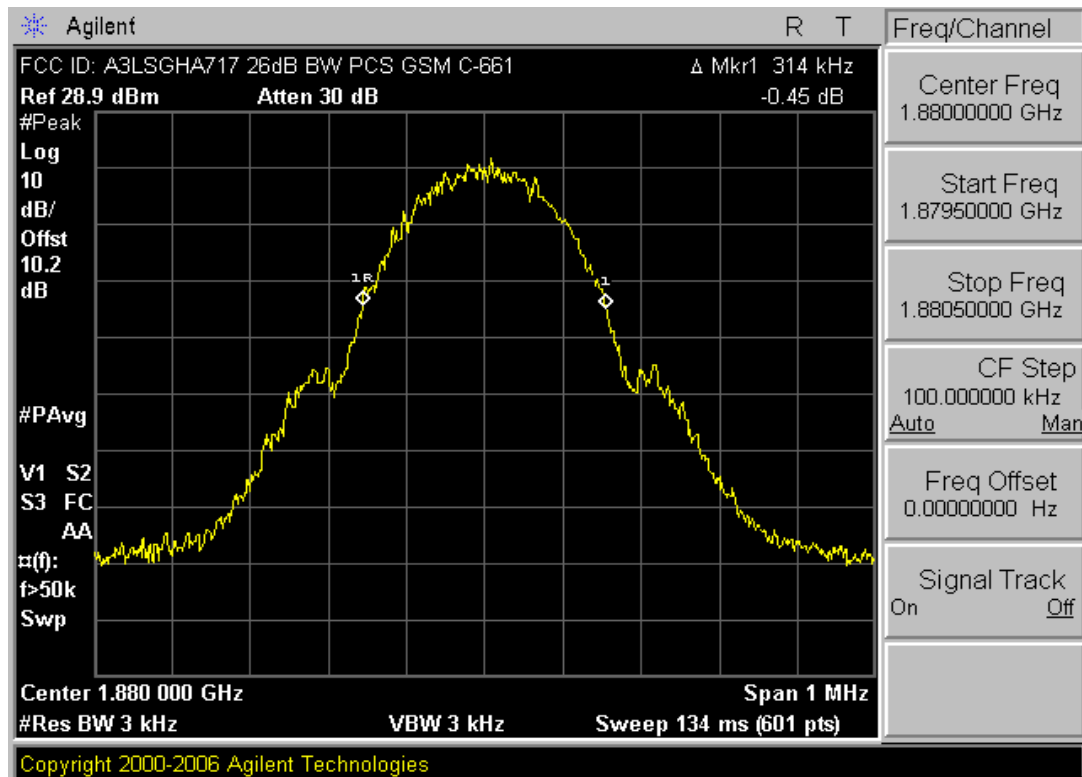
Plot 7-16. 26dB Bandwidth Plot (PCS GSM Mode – Ch. 661)
