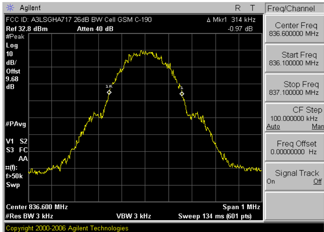
Plot 7-6. 26dB Bandwidth Plot (Cellular GSM Mode – Ch. 190)
