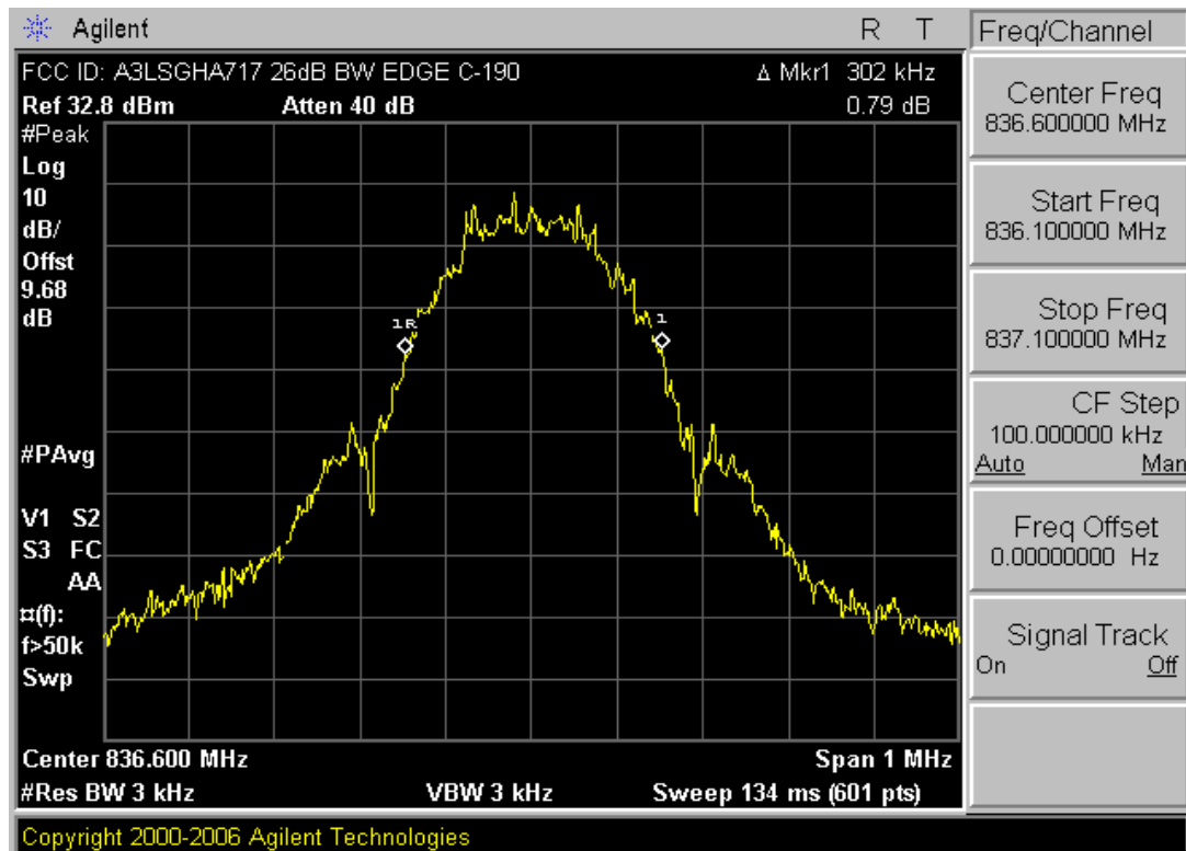
Plot 7-10. 26dB Bandwidth Plot (EDGE850 Mode – Ch. 190)
