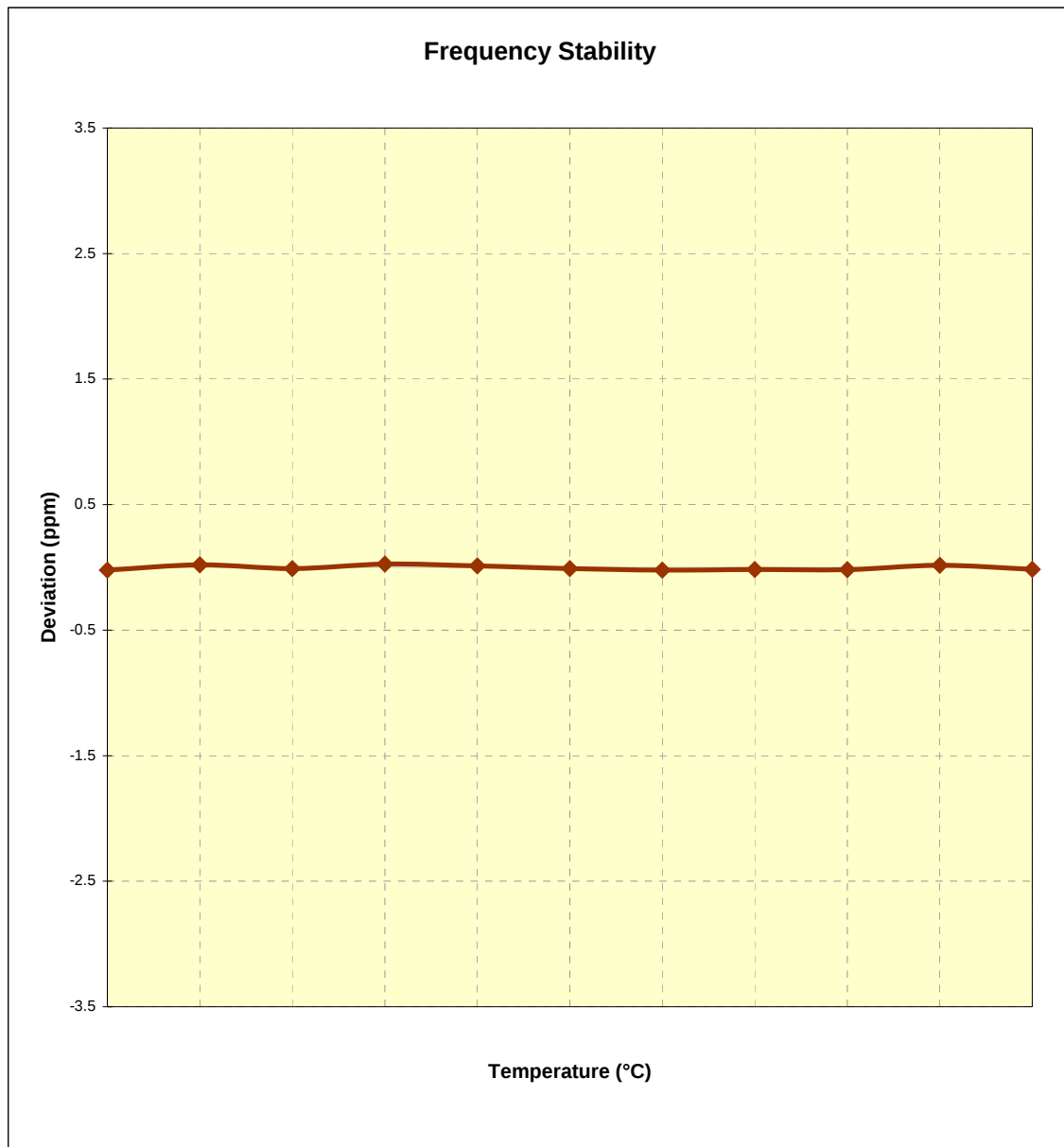
Plot 6-1. Frequency Stability Graph (Cellular WCDMA Mode – Ch. 4175)
