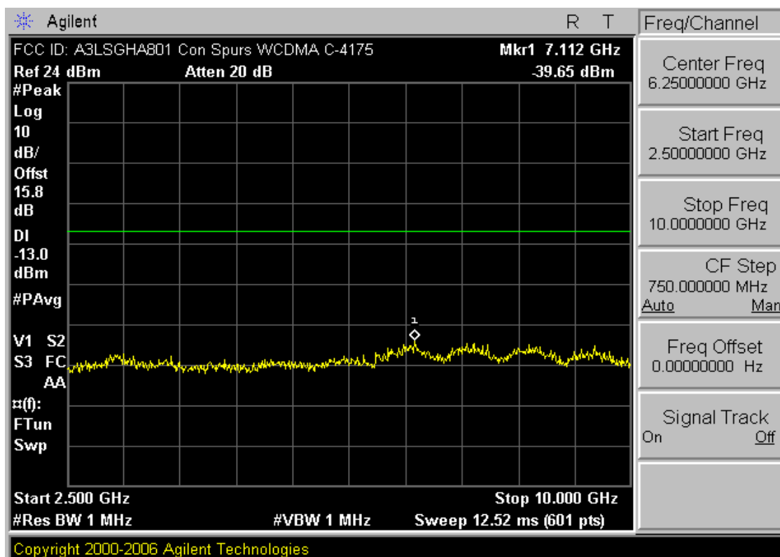
Plot 7-16. Conducted Spurious Plot (Cellular WCDMA Mode – Ch. 4175)
