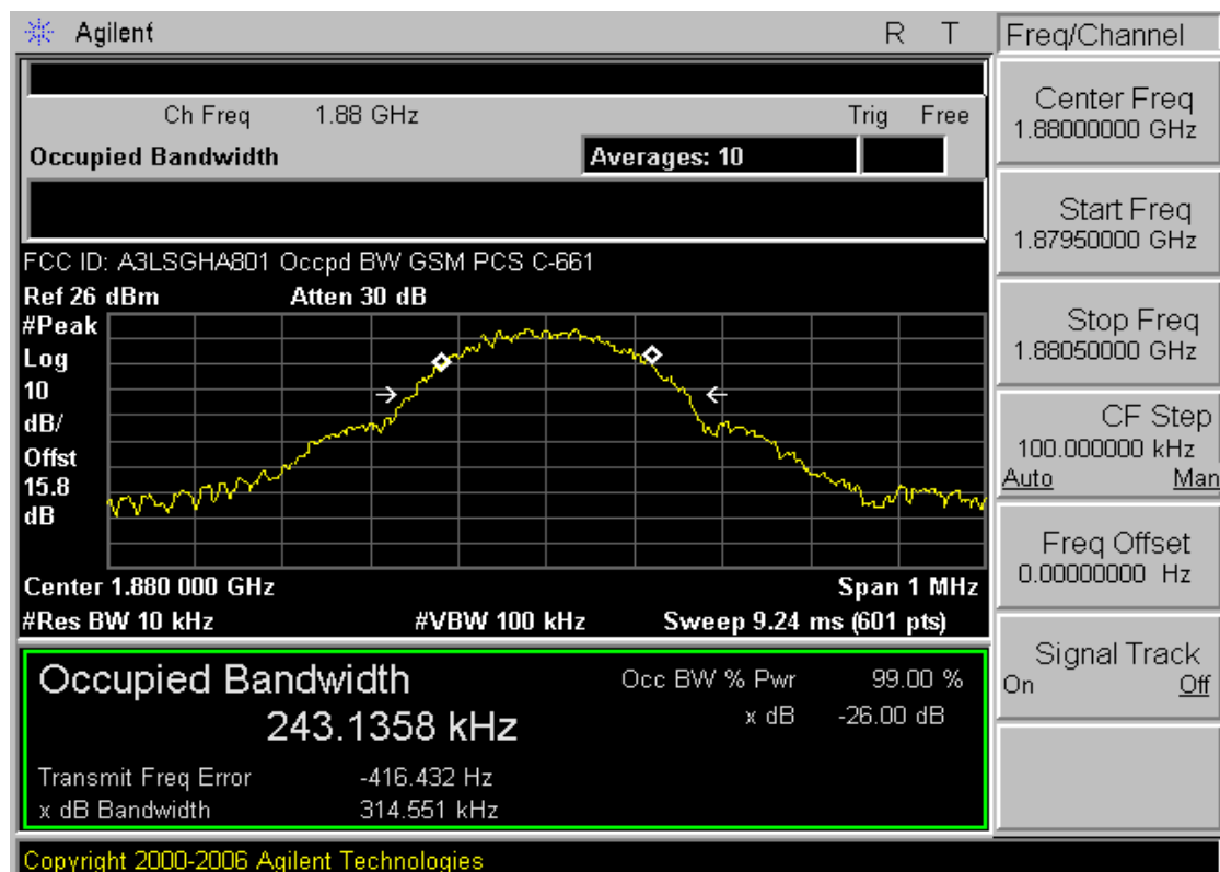
Plot 7-10. Occupied Bandwidth Plot (EDGE1900 Mode – Ch. 661)
