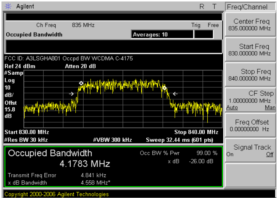
Plot 7-17. Occupied Bandwidth Plot (Cellular WCDMA Mode – Ch. 4175)
