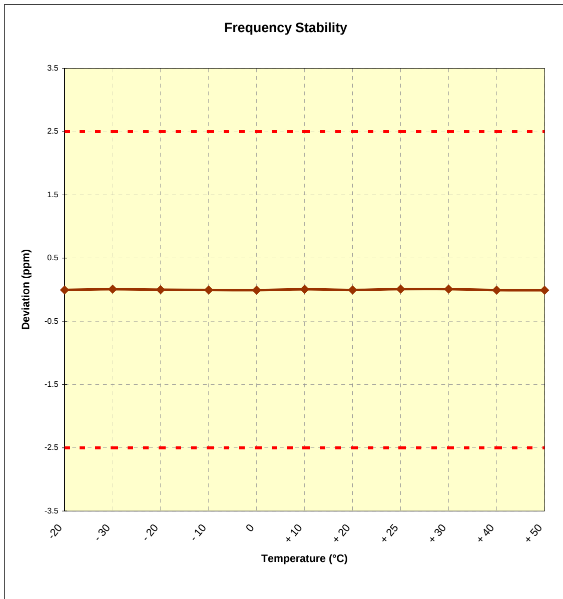
Plot 6-2. Frequency Stability Graph (PCS GSM Mode – Ch. 661)
