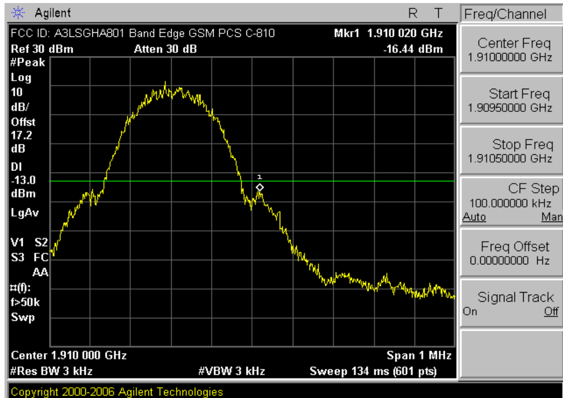
Plot 7-9. Band Edge Plot (PCS GSM Mode – Ch. 810)
