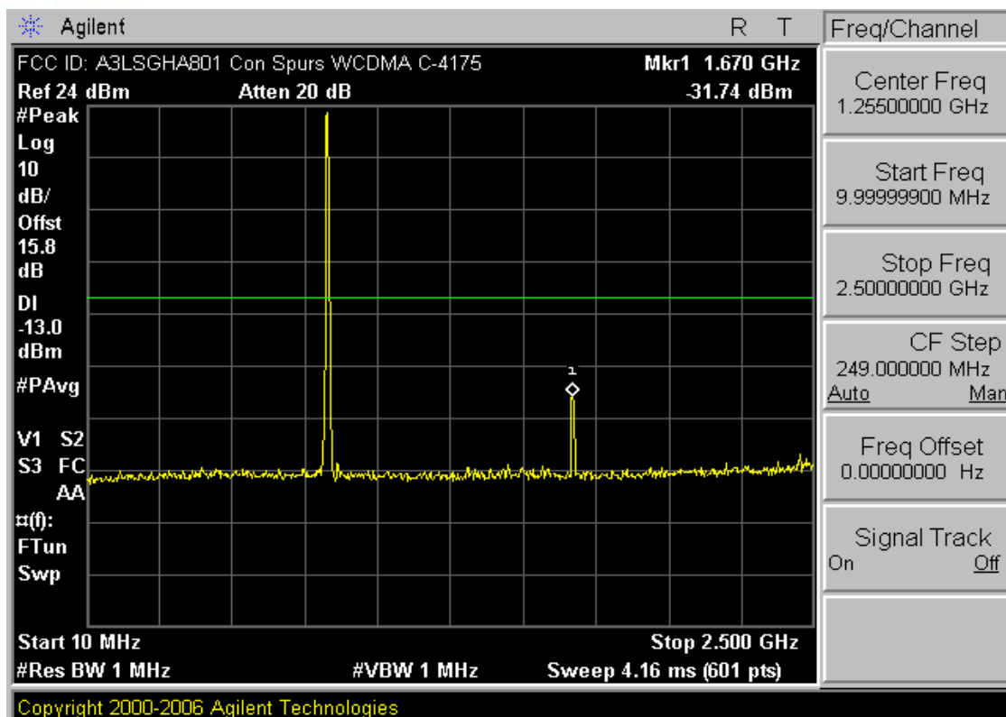
Plot 7-15. Conducted Spurious Plot (Cellular WCDMA Mode – Ch. 4175)
