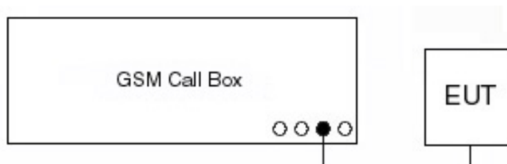
Figure 6-1. GSM Conducted Power Test Setup Diagram
