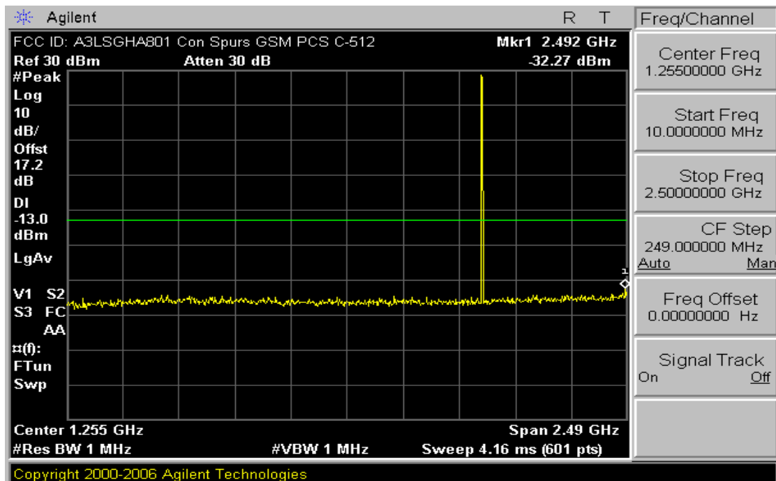
Plot 7-1. Conducted Spurious Plot (PCS GSM Mode – Ch. 512)
