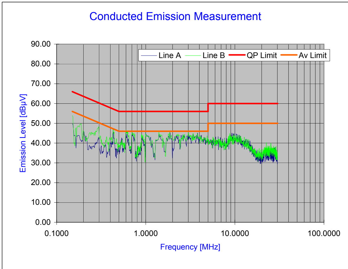
Plot 7-1. Line-Conducted Test Plot
