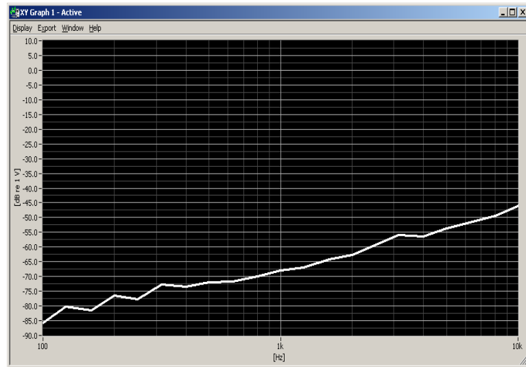
Figure 7-2 Worst-case ABM2 Plot for WD
